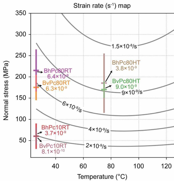
Bv: bedding-vertical; Bh: bedding-horizontal Pc: confining pressure, MPa RT: room temperature (26°C) HT: high temperature (75°C) color bars: strain rates during the pressure solution creep period
