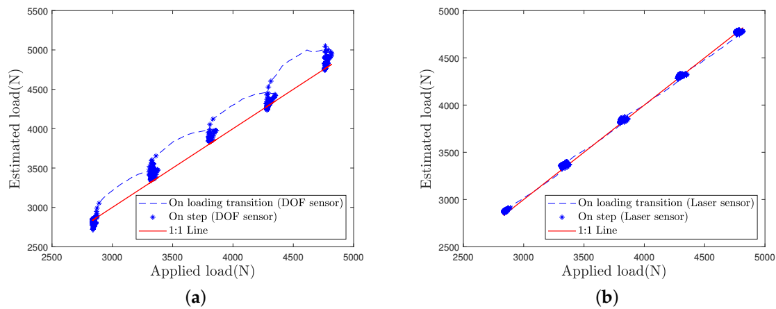
Figure 18. Load estimation for the L_{500} test case: (a) DOF sensor (b) Laser sensor.
