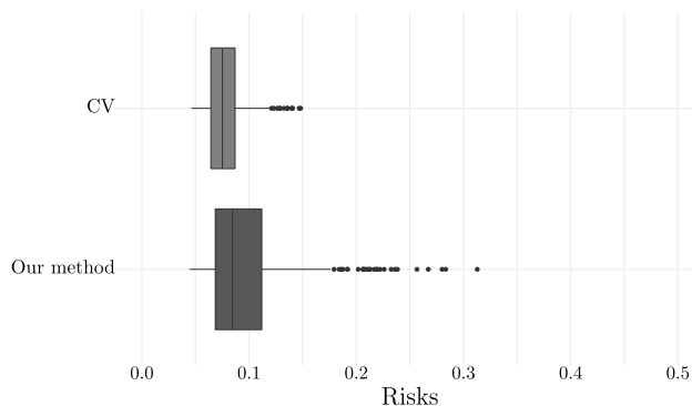
FIG 5. CV versus our method: comparing the pointwise risk \mathcal{R}(\hat{X}; 0.5) for smoothing the noisy trajectories of a fBm; simulation (1, 1000, 500, 300, equi , 0.5, 0.05).
