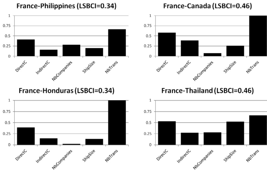
FIGURE 7. CONFIGURATIONS OF INDIVIDUAL COMPONENTS ON PAIRS OF SERVICES WITH IDENTICAL LSBCI SCORES (2016 DATA).
