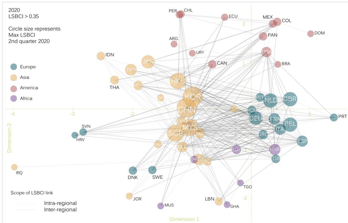
FIGURE 3. MDS VISUALIZATION OF THE LSBCI. DIMENSIONS 1 AND 2. COUNTRIES INVOLVED IN TOP LINKS (LSBCI>0.35)
