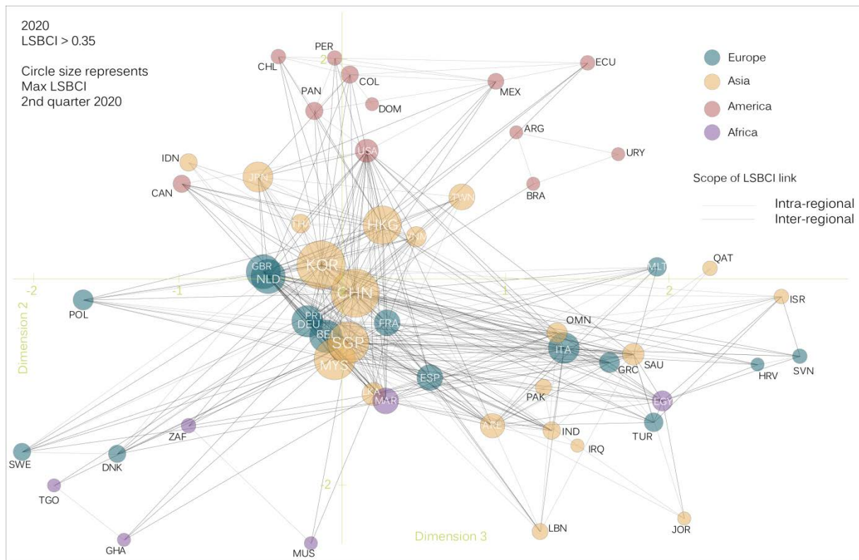
FIGURE 4. MDS VISUALIZATION OF THE LSBCI. DIMENSIONS 3 AND 2. COUNTRIES INVOLVED IN TOP LINKS (LSBCI>0.35)
