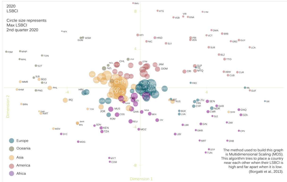
FIGURE 2. MDS VISUALIZATION OF THE LSBCI. DIMENSIONS 1 AND 2. ALL COUNTRIES
