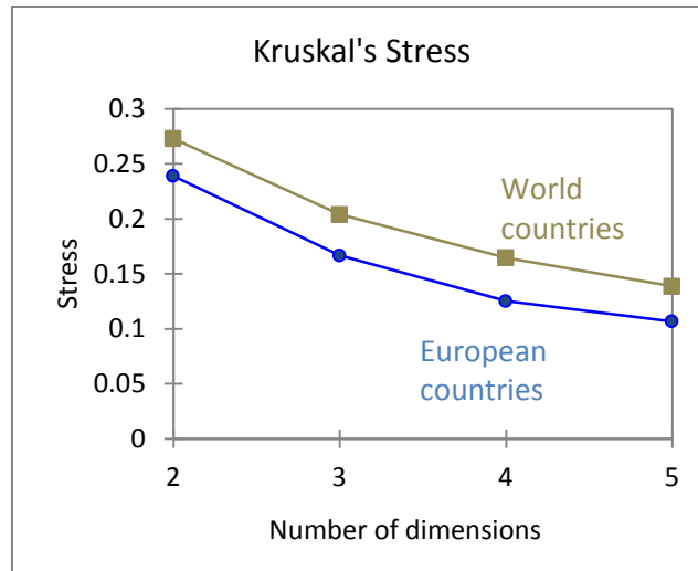
FIGURE 1. MDS KRUSKAL'S STRESS
