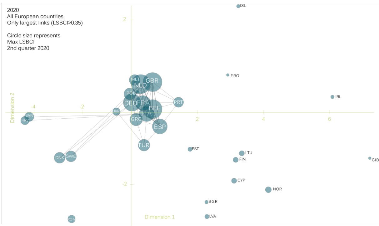
FIGURE 5. MDS VISUALIZATION OF THE LSBCI BETWEEN EUROPEAN COUNTRIES. DIMENSIONS 1 AND 2. STRESS: 0.24
