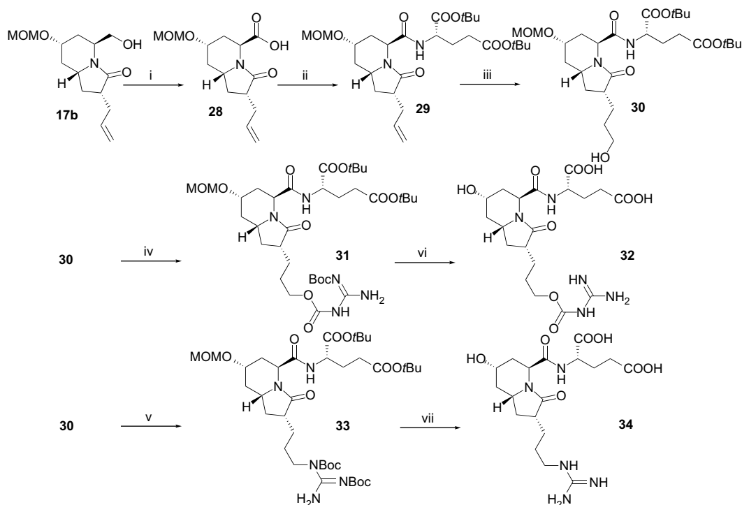
Scheme 4. Functionalization of the trans diastereoisomer: (i) \text{CrO}_3 , \text{H}_2\text{SO}_4 , acetone, 0^\circ\text{C} , 40 min, 54%; (ii) NMM, \text{ClCOOtBu} , L-Glu(O t Bu)-O t Bu, \text{CH}_2\text{Cl}_2 , 90%; (iii) (a) 9-BBN; (b) \text{H}_2\text{O}_2 , AcONa, 65%; (iv) ADPP, \text{PBu}_3 , di-Boc-guanidine, THF, reflux, 2 h, 43%; (v) DEAD, \text{PPh}_3 , di-Boc-guanidine, THF, rt, 64 h, 60%; (vi) TFA, \text{CH}_2\text{Cl}_2 , 100%; (vii) TFA, \text{CH}_2\text{Cl}_2 , 100%.
