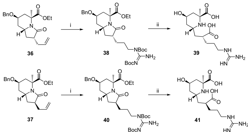
Scheme 6. Functionalization and hydrolysis of the trans diaxial diastereoisomer: (i) (a) 9-BBN; (b) \text{H}_2\text{O}_2 , AcONa; (c) DEAD, \text{PPh}_3 , di-Boc-guanidine, THF, rt ( 38 , 54%; 40 , 87%); (ii) EtOH/ \text{H}_2\text{O} , HCl 3 M, 100%.
