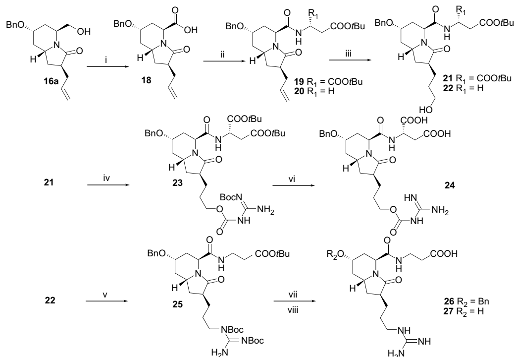
Scheme 3. Functionalization of the cis diastereoisomer: (i) \text{CrO}_3 , \text{H}_2\text{SO}_4 , acetone, 0^\circ\text{C} , 40 min, 67%; (ii) NMM, \text{ClCOOtBu} , L-BAla-O t Bu or L-Asp(O t Bu)-O t Bu, \text{CH}_2\text{Cl}_2 , \text{R}_1=\text{H} , 83%, \text{R}_1=\text{COOtBu} , 88%; (iii) (a) 9-BBN; (b) \text{H}_2\text{O}_2 , AcONa, \text{R}_1=\text{COOtBu} , 68%, \text{R}_1=\text{H} , 71%; (iv) ADPP, \text{PBu}_3 , di-Boc-guanidine, toluene, reflux, 2 h, 60%; (v) DEAD, \text{PPh}_3 , di-Boc-guanidine, THF, rt, 64 h, 92%; (vi) TFA, \text{CH}_2\text{Cl}_2 , 100%; (vii) \text{R}_2=\text{Bn} , TFA, \text{CH}_2\text{Cl}_2 , 100%; (viii) \text{R}_2=\text{H} ; (a) \text{H}_2 Pd/C 10%, 72%; (b) TFA, \text{CH}_2\text{Cl}_2 , 100%.
