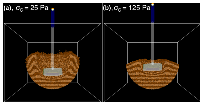
Figure 12. Using GDC-I, we simulated TAGSAM impacts into regolith with variable interparticle cohesive strength, \sigma_c . These snapshots show the simulation state 2.7 s after contact. (a) Regolith with \sigma_c = 25 \text{ Pa} provides little resistance to TAGSAM. (b) Regolith with \sigma_c = 125 \text{ Pa} can effectively limit TAGSAM penetration.
