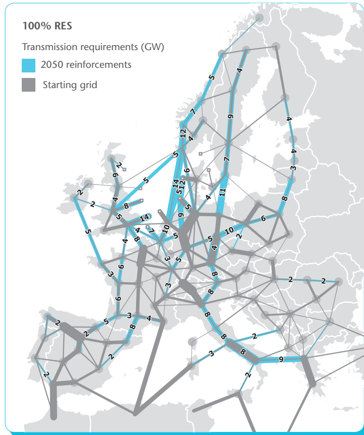
Figure 4.1. Transmission requirements identified in a scenario of 100% RES by 2050, in GW
