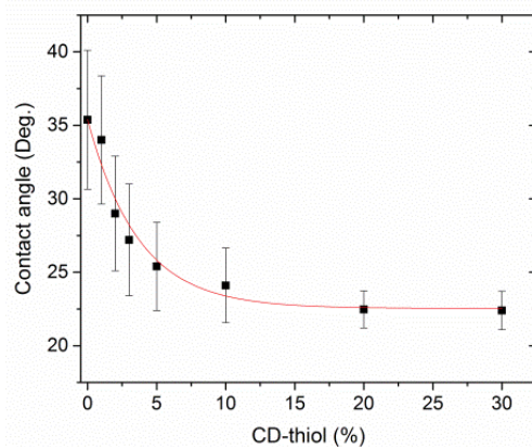
Figure S1. Contact angle of water on \beta -CD SAMs as a function of the molar ratios of CD-thiol in the solution used to prepare the \beta -CD SAMs.
