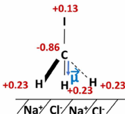
Figure 3 Scheme of CH 3 I monomer adsorption on NaCl and Mulliken charge distribution calculated with DFT performed using \omega B97XD/aug-cc-pVTZ-PP level of theory.
