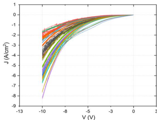
Figure 3. Surface normalization of reverse current (23 diodes with diameters ranging from 40 to 2 \mu m)
