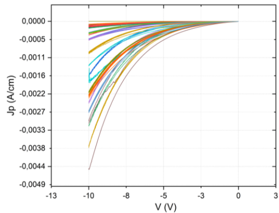
Figure 4. Perimeter normalization of reverse current (23 diodes with diameters ranging from 40 to 2 \mu m)
