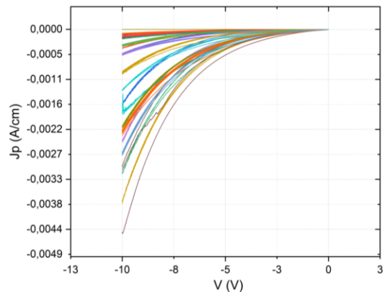
Figure 4. Perimeter normalization of reverse current (23 diodes with diameters ranging from 40 to 2 \mu\text{m} )
