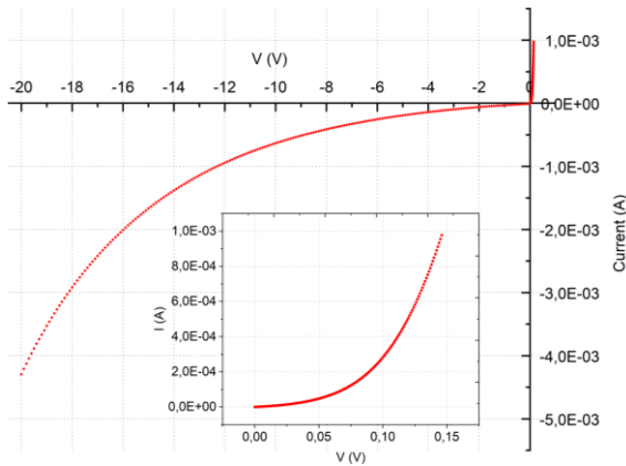
Figure 2. I-V characteristic of a 70 \mu m diode (inset: forward characteristic)
