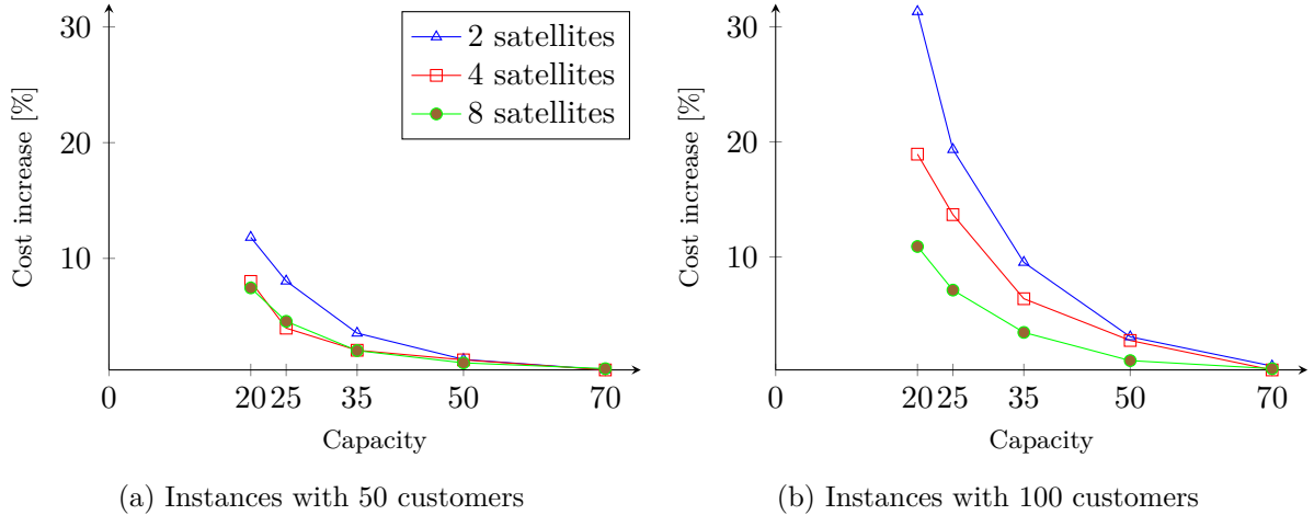
Figure 8: Average cost increase (in percent) compared to the respective instance with infinite satellite capacity
