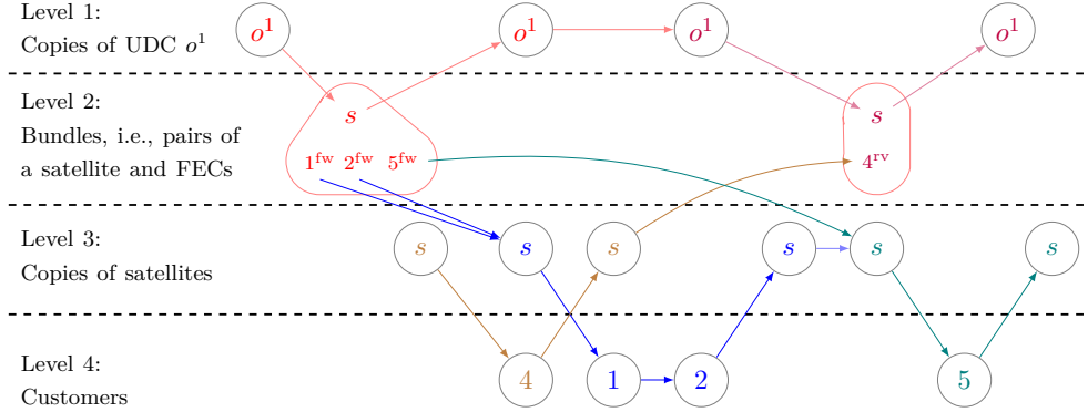
(c) Representation with precedence graph
