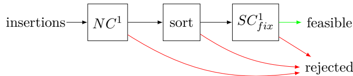
Figure 4: Sequence of necessary and sufficient conditions in the feasibility test of LNS 1
