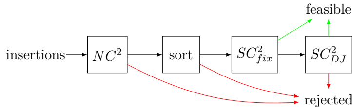
Figure 5: Sequence of necessary and sufficient conditions in the feasibility tests of LNS 2
