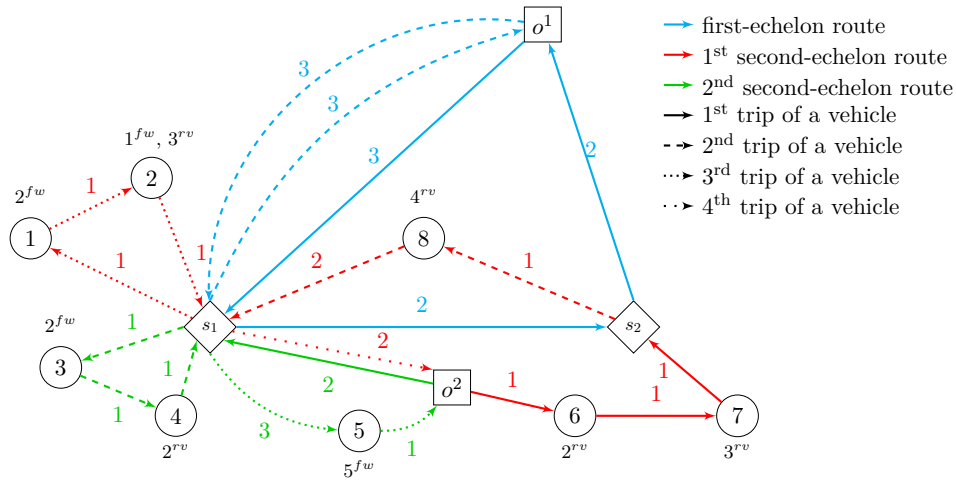
Figure 1: 2E-MTVRP-CSRFP solution used in Example 1
