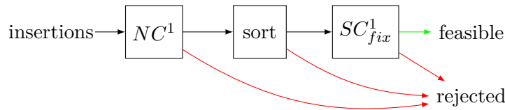
Figure 4: Sequence of necessary and sufficient conditions in the feasibility test of LNS 1
