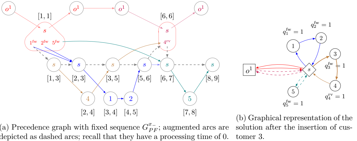
Figure 6: Insertion of customer 3 into the second-echelon trip (s, 4, s) , continued from Example 2; the new solution is temporal feasible
