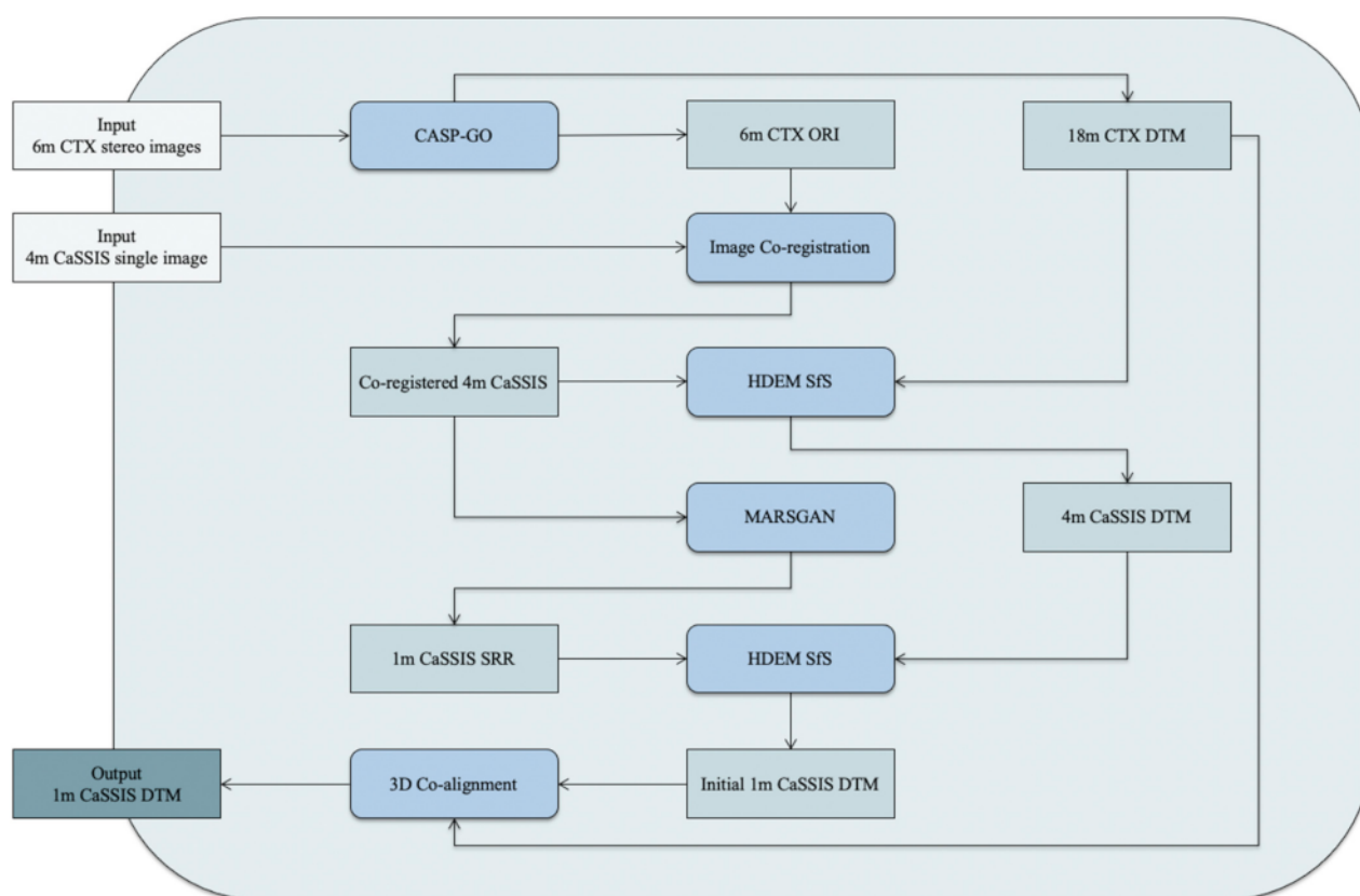
Figure 2. Flow diagram of the proposed ultra-high-resolution CaSSIS DTM processing system.
