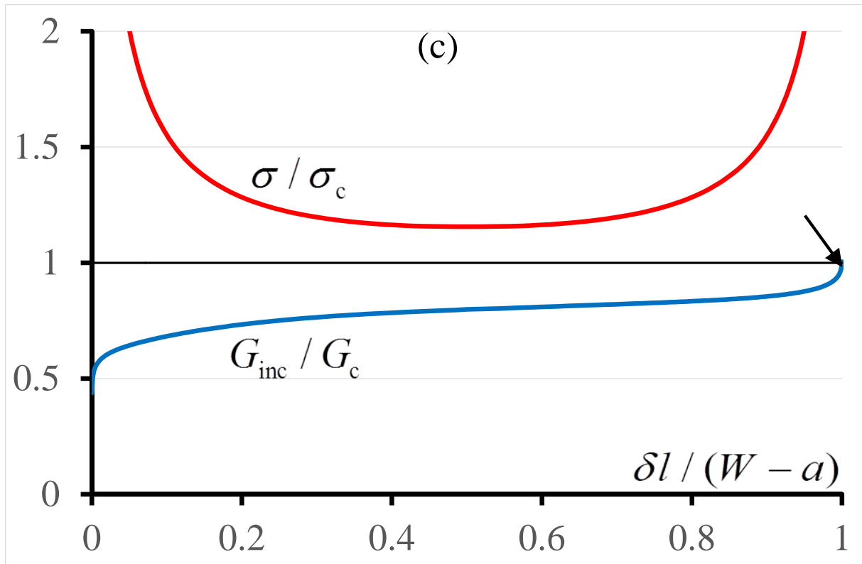
Figure 1. Examples of implementation of the CC. (a) The U-notched specimen at the \mu -scale under FC loading (Section 3.5). (b) The U-notched specimen at the \mu -scale under DC loading (Section 3.5). (c) The double edge notched specimen at the nm-scale under DC loading (Section 4.3). Stress condition (10): red solid line, energy condition (8): blue solid line. The horizontal axis is the crack length normalized by the ligament width. The arrow shows the point that meets the two conditions. Refer to Section 3 for DC and FC meaning.
