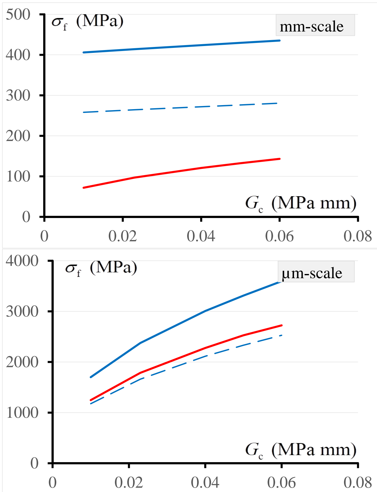
Figure 8. The stress \sigma_f function of the fracture energy G_c at the mm-scale and the \mu m-scale for the U-notched specimen with \rho=0.02 (red solid line), for the plain specimen with height W = 2 (blue solid line) and for the plain specimen with height W - a = 1.6 (blue dashed line). Computations are carried out under FC loading.
