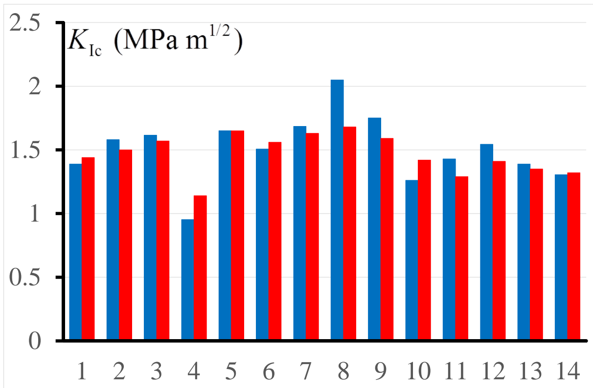
Figure 11. Comparison on the identification of the material toughness K_{Ic} between the present analysis (blue) and Henry et al. [35] estimates (red) for the 14 specimens.
