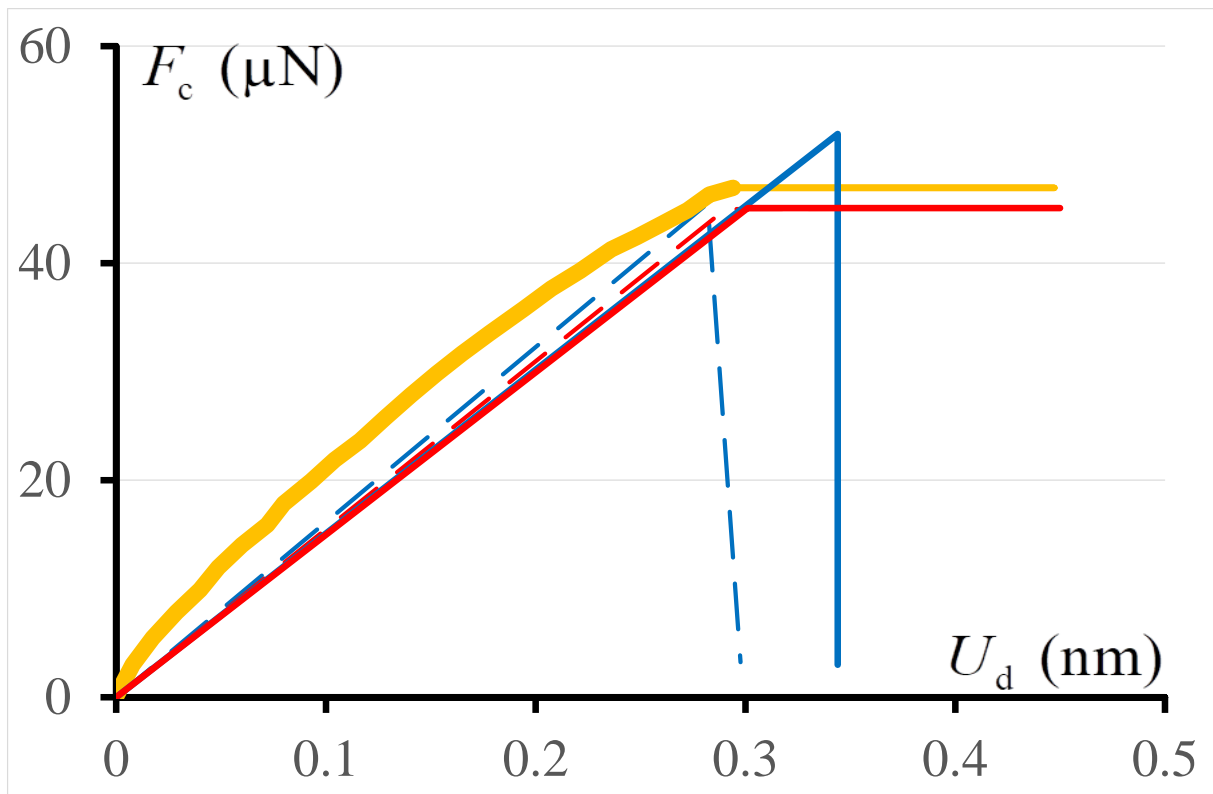
Figure 17. Simulation of failure of the nano-platelet of aragonite. MD: orange solid line, PF under DC loading: blue dashed line, PF under FC loading: red dashed line, CC under DC: blue solid line, CC under FC: red solid line. Results are obtained with \sigma_c = 5 GPa.
