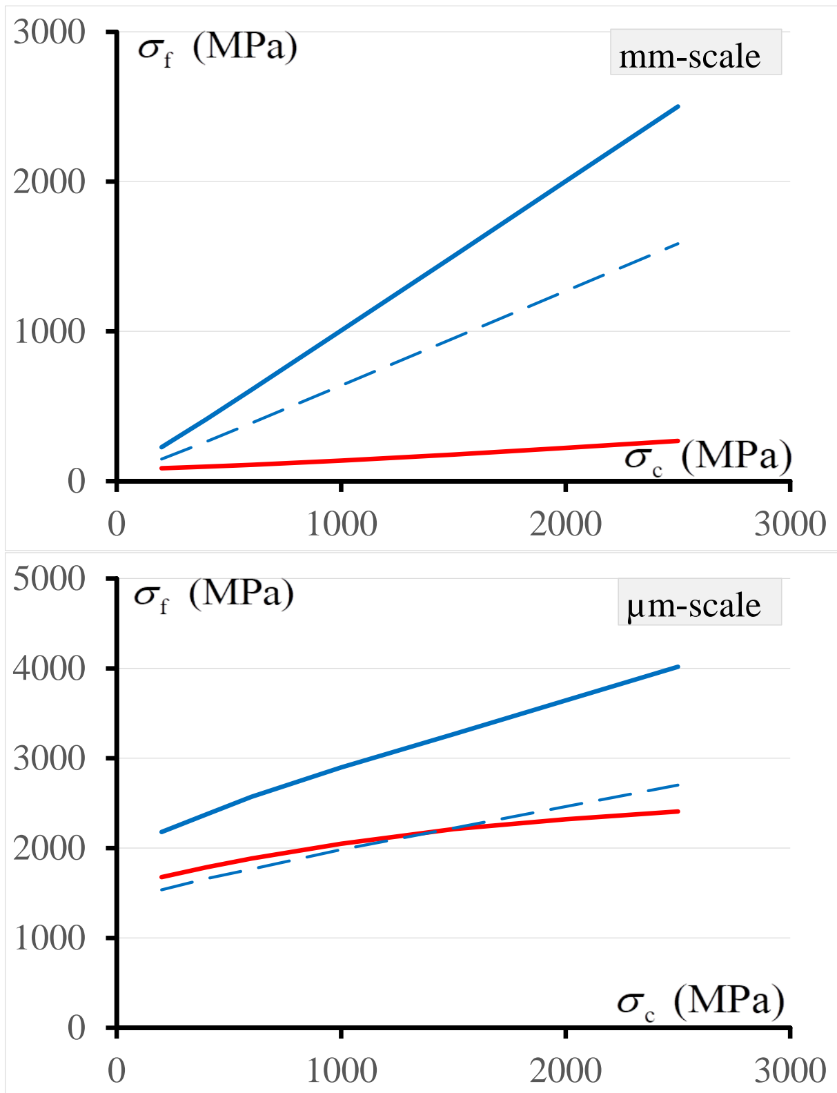
Figure 9. The stress \sigma_f function of the tensile strength \sigma_c at the mm-scale and the \mu m-scale for the U-notched specimen with \rho = 0.02 (red solid line), for the plain specimen with width W = 2 (blue solid line) and for the plain specimen with width W - a = 1.6 (blue dashed line). Computations are carried out under FC loading mode.
