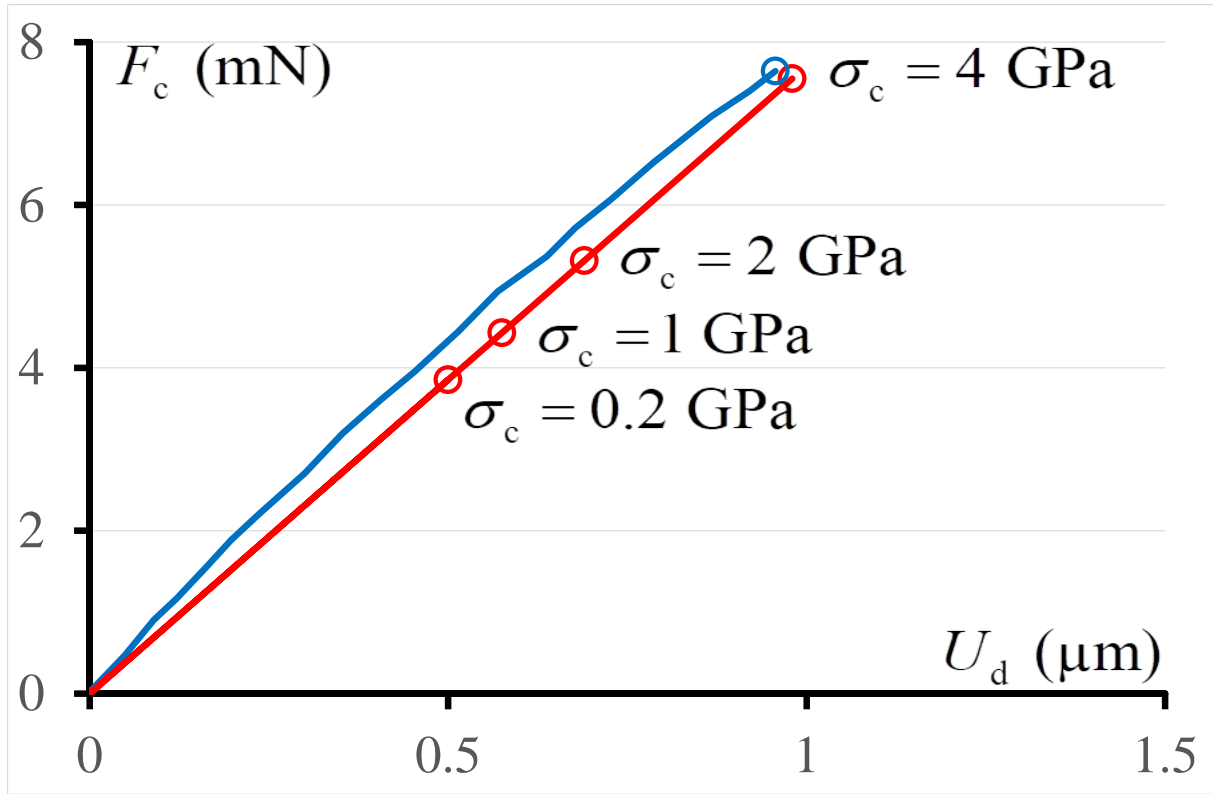
Figure 14. The applied force at failure function of the prescribed displacement. The blue solid line is the loading curve, the red solid one is the simulated one. The blue circle corresponds to the specimen failure in the experiments. The red circles are the failure loads predicted by the CC for various tensile strength values \sigma_c .
