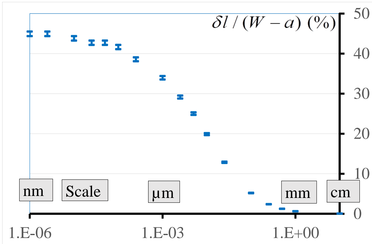
Figure 5. The ratio \delta l / (W - a) at various scales for \omega = 90 deg. (FC loading). The error bars correspond to the mesh size.
