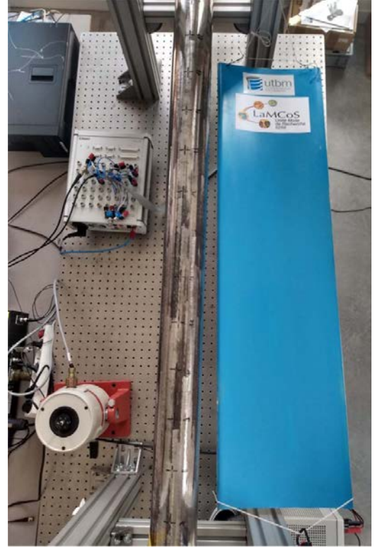
Figure 3. Smart composite structure: top view.
