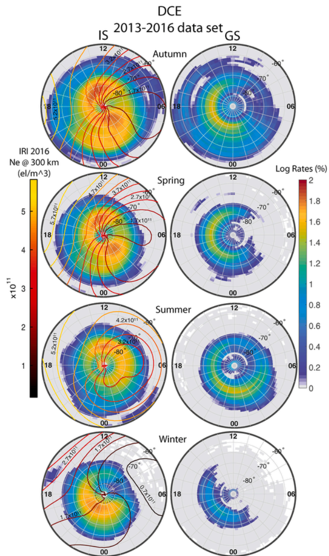
Fig. 3. Dome C East ionospheric scatter (IS), left column, and ground scatter (GS), right column, Echo Occurrence (EO) rates for the 2013–2016 dataset plotted in MLT- MLAT coordinates. The maps from top to bottom are for Autumn, Spring, Summer and Winter, respectively. The GS rate maps are for the same periods. Noon MLT is at the top of the maps, dawn (6 MLT) is to the right and dusk (18 MLT) is to the left. The EO rates are expressed as logarithm of percents (the rate of 1 corresponds to 100 percent) according to the logarithmic colour scale on the right. The contours of the beam averaged electron density at 300 km are overplotted on the IS maps. The contours are coloured according to the scale on the left of the figure. The electron density is derived from the IRI-2016 model for equinoxes and solstices of 2013 as described in the text. (For interpretation of the references to colour in this figure legend, the reader is referred to the Web version of this article.)
