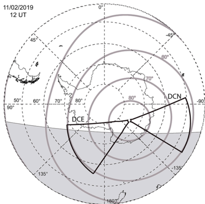
Fig. 1. The Dome C East (DCE) and Dome C North (DCN) radars Fields of View for February 11, 2019, 12 UT. The geographic coordinates system is represented by dashed lines. The AACGM magnetic latitudes are shown by solid grey lines. Solar noon is at the top, midnight at the bottom. The shaded region is the Earth's portion in darkness.
