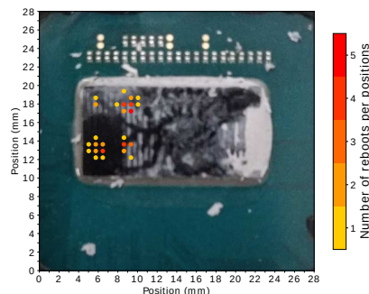
Figure 3: Probe positions over the Intel Core i3 where the system is sensitive to fault.
