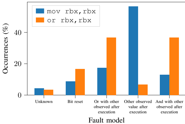
Figure 4: Fault models distribution and their probability of occurrence on the Intel Core i3-6100T perturbed with EMFI.
