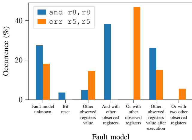
Figure 2: Fault models distribution and their probability of occurrence on the BCM2837 perturbed with EMFI.
