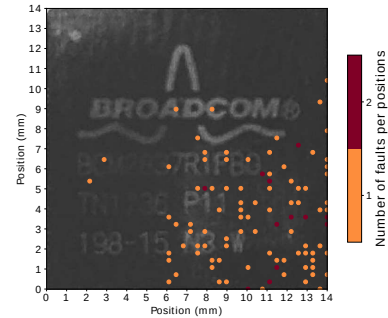
Figure 1: Probe positions over the BCM2837 leading to faults.
