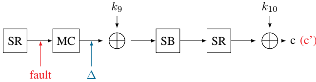
Figure 5: DFA Principle
