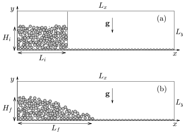
FIGURE 2. Sketch of the 3D setup in a 2D streamwise (x, y) plane at a fixed z coordinate. Unit vector \mathbf{z} is in the out of plane direction. (a) initial configuration at t = 0 and (b) final deposit for t \geq t_f .
