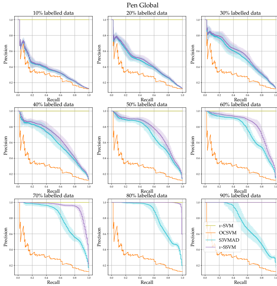
Figure 5: Mean PR curves for various percentages of labeled data - Pen Global dataset.
