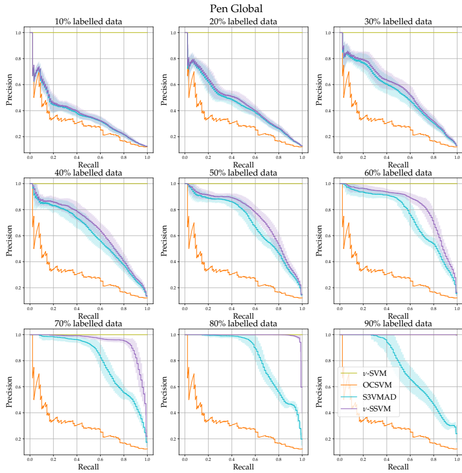
Figure 5: Mean PR curves for various percentages of labeled data - Pen Global dataset.
