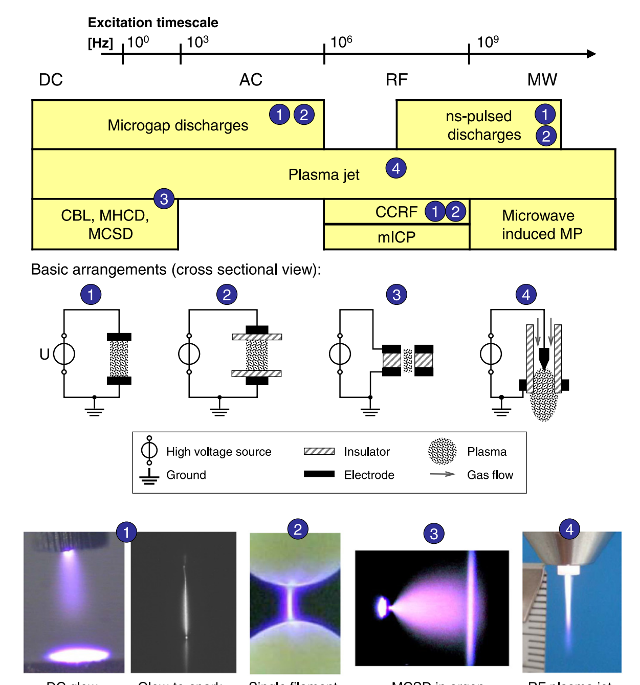
Figure 2. Microplasma arrangements categorized by excitation timescale and basic electrode geometry. The images in the bottom part of the figure represent a dc excited stable glow discharge [66] © IOP, a partly contracted glow discharge (with clearly a visible anode and cathode spot) during a glow-to-spark transition [65] © IOP, a semi-spherical volume DBD with a single filament as described in [136], a side-on view of a MHCD (left) and the MCS glow discharge (right) [83] © AIP, and an RF-driven plasma jet as described in [230]. The images are reproduced with permission from IOP, AIP and IOP/Greifswald, respectively. The abbreviations are explained in detail in the text.
