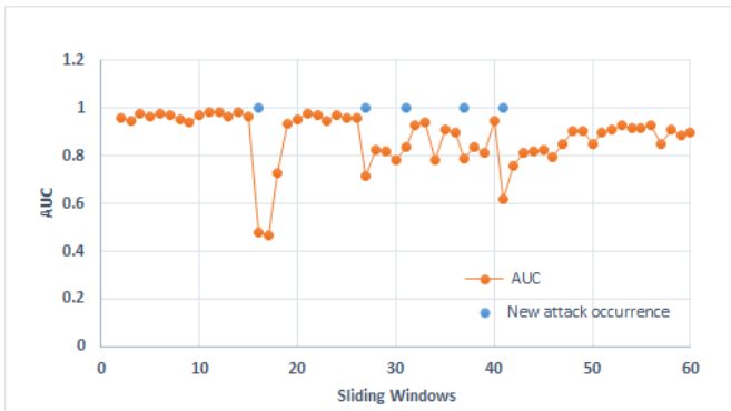
Fig. 3. Results of the incremental and active learning-based IDS on the different sliding windows
