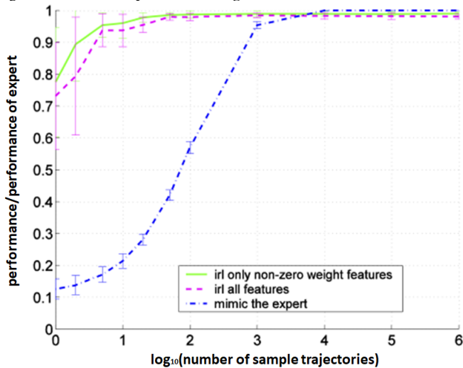
Fig. 1. Ideal IRL Experiments using Frame/Grid Like data instances
