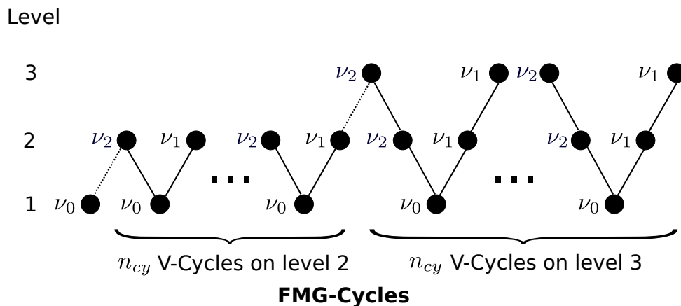
Figure 2: FMG cycles
