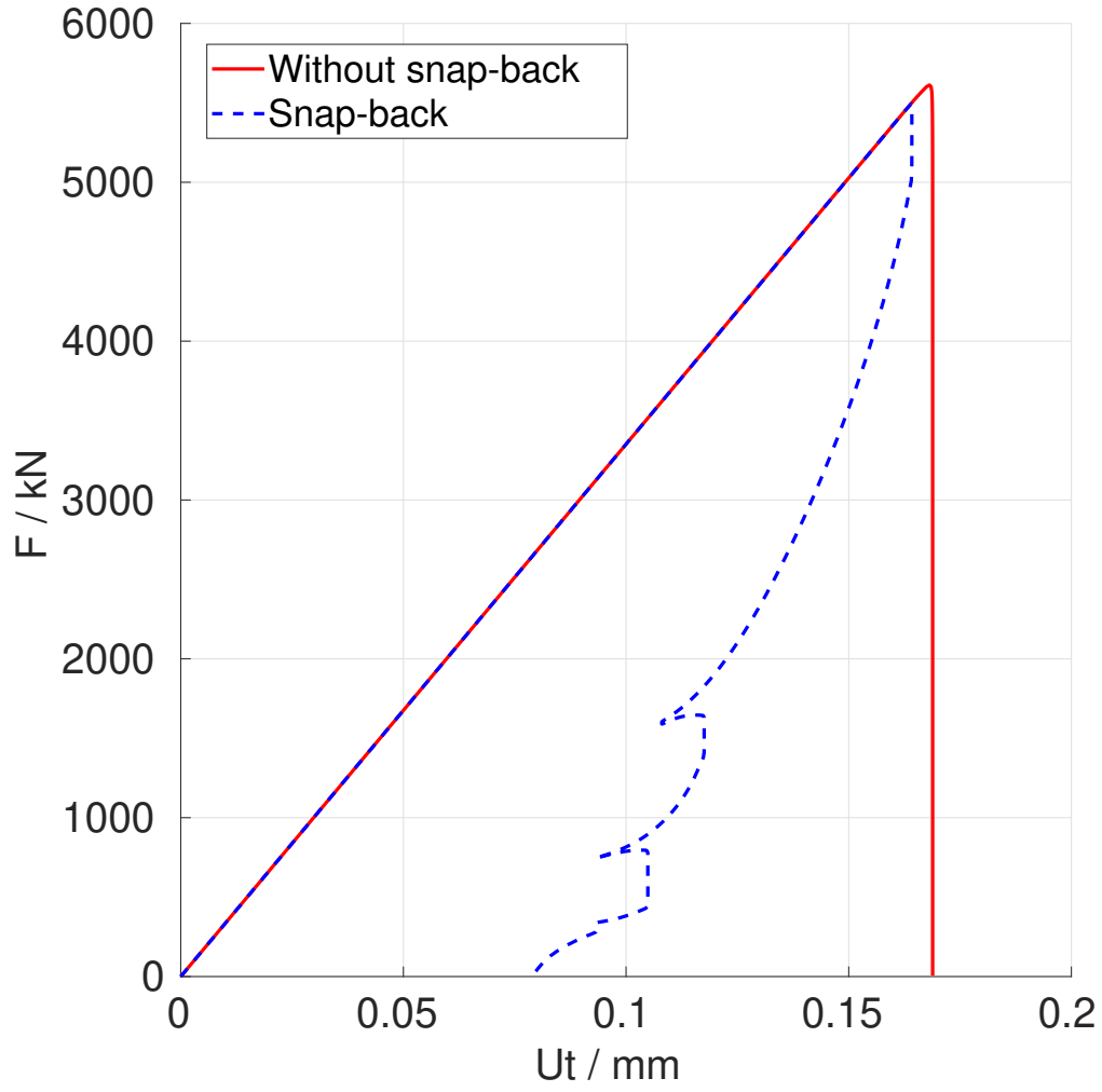
Figure 15: Snap-back behavior
