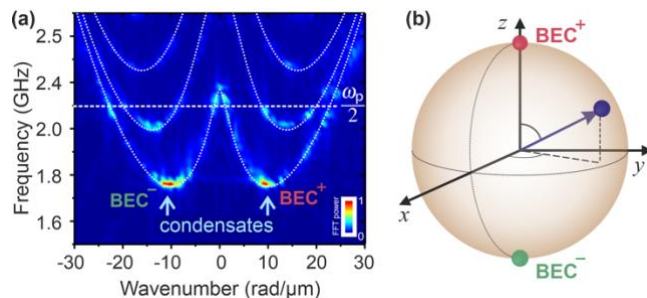
Fig. VIII.A. (a) Numerical simulation of the condensation process in a parametrically populated magnon gas (adapted under the terms of the Creative Commons Attribution 4.0 licence from [399]) leading to a qubit state lying on the equator of the Bloch sphere shown in panel (b). (b) Representation of a magnon BEC qubit (blue dot) on the surface of a Bloch sphere. The BEC^+ (North Pole) and BEC^- (South Pole) states are indicated by the red and green dots.
