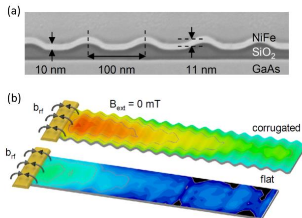
Fig. III.F. (a) Transmission electron microscopy image of the cross-section of the corrugated waveguide. The corrugation induces the effective anisotropy field of 5 mT perpendicular to the corrugation direction. (b) Comparison of zero-field spin-wave propagation in the corrugated and a flat reference waveguide, imaged by micro-BLS. Corrugation-induced anisotropy stabilizes magnetization perpendicularly to the waveguide's long axis. The spin waves then propagate in the most favorable Damon-Eshbach geometry, with high group velocity, over a distance 10× larger than in the flat reference waveguide. Reproduced from [171]; licensed under a Creative Commons Attribution (CC BY) license.
