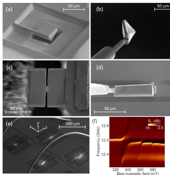
Fig. 8B1. (a)–(e) FIB fabrication steps of YIG-on-superconductor samples [402]. (f) Ultra-strong coupling evidence obtained at 80 mK for the structure shown in (e) together with theoretical calculation based on [403] (Reproduced from [402], with the permission of AIP Publishing).
