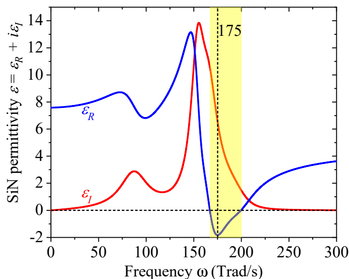
Figure 2. Real and imaginary parts of the relative permittivity \varepsilon = \varepsilon_R + i\varepsilon_I of SiN, as a function of frequency [23]. The yellow zone stands for the band in which \varepsilon_R < 0 .
