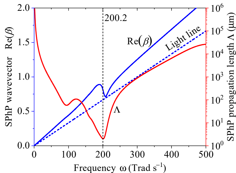
Figure 3. Frequency spectrum of the wavevector and propagation length of SPhPs propagating along a SiN nanowire suspended in air ( \varepsilon_0 = 1 ). The blue dashed line stands for the wavevector of light in vacuum.
