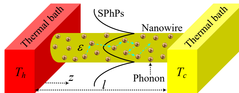
Figure 1. Scheme of a polar nanowire supporting the propagation of both SPhPs and phonons due to the temperature difference T_h > T_c imposed by two thermal baths.
