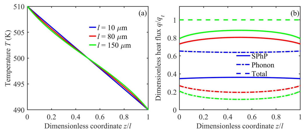
Figure 4. (a) Temperature and (b) heat flux profiles in a SiN nanowire with representative lengths l . The solid and dashed-dot lines in (b) represent the respective SPhP and phonon heat fluxes, whereas the dashed one stands for the total heat flux q_t . Calculations were carried out for a SiN nanowire with a radius a = 50 \text{ nm} and a typical phonon thermal conductivity of k_{ph} = 1 \text{ W/m}\cdot\text{K} .
