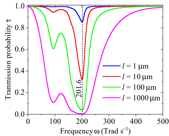
Figure 5. Frequency spectrum of the transmission probability of SPhPs propagating along a SiN nanowire of different lengths.
