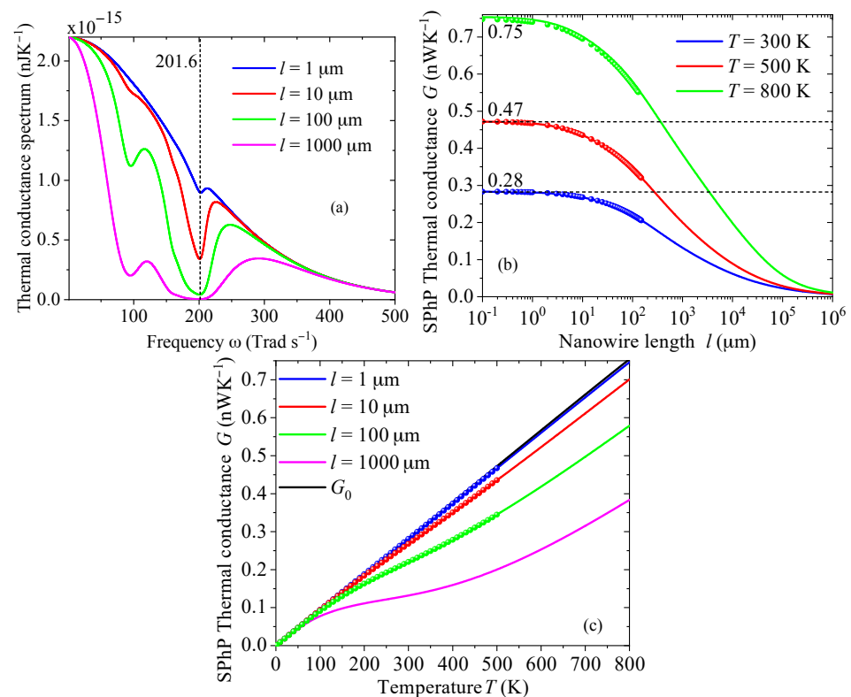
Figure 6. (a) SPhP thermal conductance spectrum along with its integrated counterpart as a function of the (b) length and (c) temperature of a SiN nanowire suspended in air with a radius a = 50 \text{ nm} . The solid lines represent the predictions of Equation (17) and the dots the stand for the numerical results obtained with the DOM+FDMM described in Section 2.1. Calculations in (a) were carried out for T = 300 \text{ K} .
