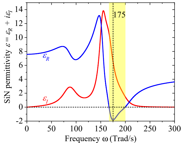
Figure 2. Real and imaginary parts of the relative permittivity \varepsilon = \varepsilon_R + i\varepsilon_I of SiN, as a function of frequency [23]. The yellow zone stands for the band in which \varepsilon_R < 0 .
