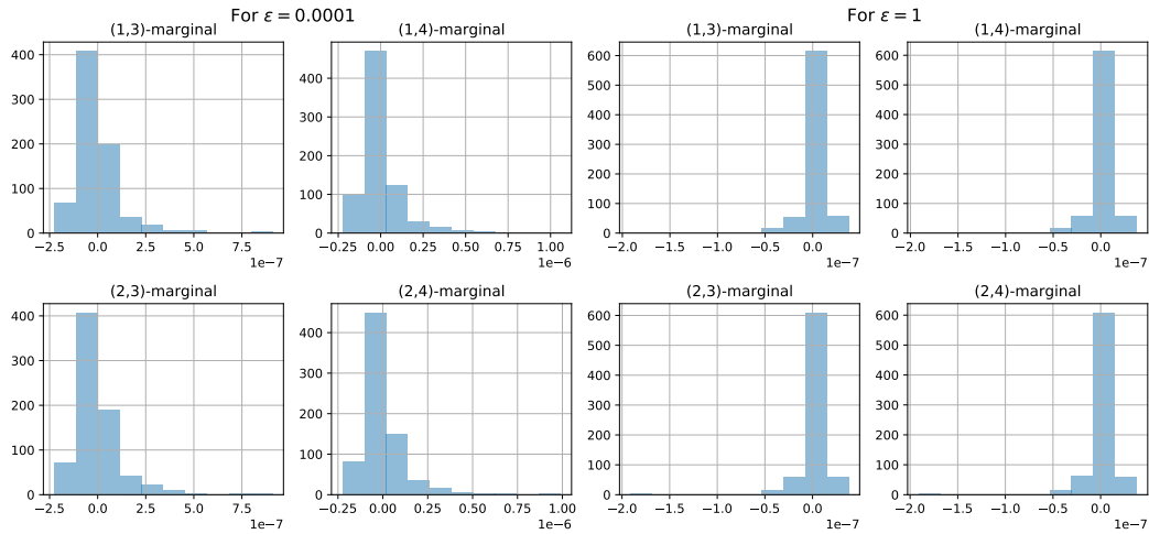
Figure 2: Histograms of difference between true independent marginal matrices and their approximations. We see that the marginal matrices obtained by the algorithm 1 approximate well the theoretical uniform matrices.
