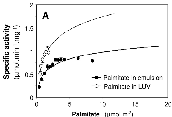
Figure 5. Variation in FAPv2 specific activity ( \mu\text{mol} \cdot \text{min}^{-1} \cdot \text{mg}^{-1} ) as a function of palmitate surface concentration ( \mu\text{mol} \cdot \text{m}^{-2} ) in LUV and at the surface of phospholipid-stabilized soybean oil microemulsion. The surface concentrations of PA were estimated as described in Supporting Information. Values are mean \pm SD ( n=3 ).
