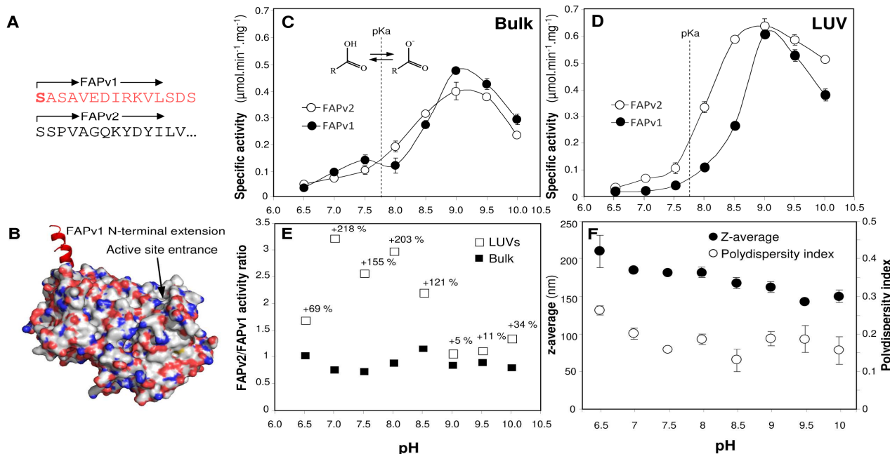
Figure 2. Comparison of the specific activities of the recombinant FAPv1 and FAPv2 variants. (A) N-terminal sequences of FAPv1 and FAPv2. The N-terminal extension present in FAPv1 and deleted in FAPv2 is indicated in red letters. Note that residue 61 in CvFAP (R) is substituted by S in FAPv1 (bold red letter) due to construct for cleavage by TeV protease. (B) 3D structure of FAPv1 showing the N-
