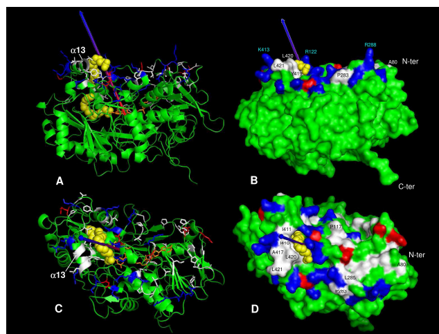
Figure 8. Interfacial Recognition Site and dipolar moment in FAPv2. Side (A, B) and top (C, D) views of FAPv2 are shown either as ribbon model with secondary structure elements (A, C) or molecular surface representation (B,D). Top views are aligned on a plateau found on one side of FAPv2, from which one co-crystallized C18 fatty acid molecule (shown as yellow spheres) emerges from the enzyme active site entrance and interacts with several residues from the amphipathic helix \alpha 13. A second fatty acid molecule is found deeper within the active site. All atoms of FAPv2 are colored in green, except those belonging to hydrophobic (white), basic (blue) and acidic (red) amino acids found in the plateau. The arrow originating from the center of gravity of the protein shows the orientation of the dipolar moment (1527 Debye) estimated for FAPv2 using a Pymol script based on an approach similar to Felder et al. (40). The blue extremity indicates the positive pole. The structure of FAPv2 is deposited in the Protein Databank under the accession number 6YRU(36).
