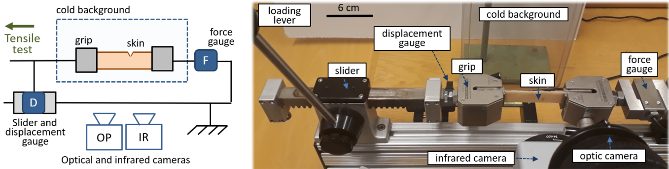
FIG. 1. Schematic (left) and picture (right) of the experimental set-up. Porcine skin is teared in front of an optical and an infrared camera, while both the applied force and displacement are measured. In the real set-up (e.g., by contrast to what is suggested by the schematic) the optical camera is placed above the infrared one.
