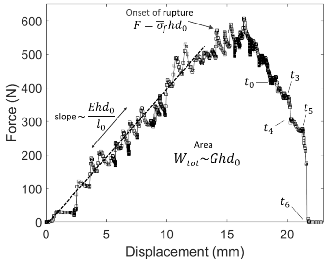
FIG. 4. Force versus displacement plot for the experiment shown in Fig. 3 (skin specimen V). Labels t_0 to t_6 refer to the times of the frames in this other figure. The relatively linear relation at small displacements allows to invert for the skin's Young modulus E . The area below the plot is the total mechanical work W_{\text{tot}} provided to the sample. The mean stress at the onset of rupture is called \bar{\sigma}_f .
