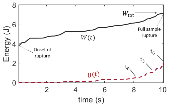
FIG. 5. (a): Comparison of the time evolution of the provided mechanical load W , as per Fig. 4, and that of the rise in internal (thermal) energy U in the skin sample, as per Eq. (4). This plot is for skin specimen V. Labels t_0 to t_6 refer to the frames of Fig. 3. The mean observable thermal efficiency, which is the ratio \phi = U/W_{\text{tot}} at the end of the rupture, is here about 30%.
