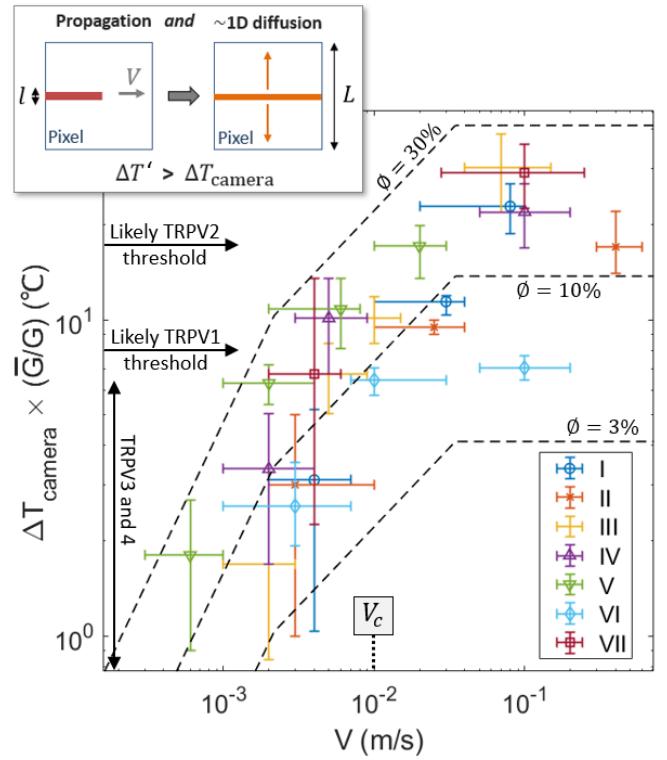
FIG. 6. Recorded elevation of temperature \Delta T at the damage tip as a function of crack velocity (log scales), scaled by \bar{G}/G for each skin sample. Data points for the seven experiments are shown with different symbols (and colours). For reference, the thresholds for the activation of the TRPVs are shown by the plain arrows, assuming an ambient temperature of 35^\circ\text{C} for live inner skin. The dashed lines are the model described by Eq. (9) using \phi = 3\% , 10\% and 30\% , and with \rho c = 3.7 \text{ MJ K}^{-1} \text{ m}^{-3} , \lambda = 0.3 \text{ J s}^{-1} \text{ m}^{-1} \text{ K}^{-1} , \bar{G} = 135 \text{ kJ m}^{-2} and l = 3 \mu\text{m} . The transition velocity V_c predicted by the model (i.e., Eq. (8)) is also indicated. The top-left inset illustrates the 1D diffusion hypothesis lying being Eq. (9), due to the time scale difference between the crack propagation and the heat diffusion at the camera pixel size.
