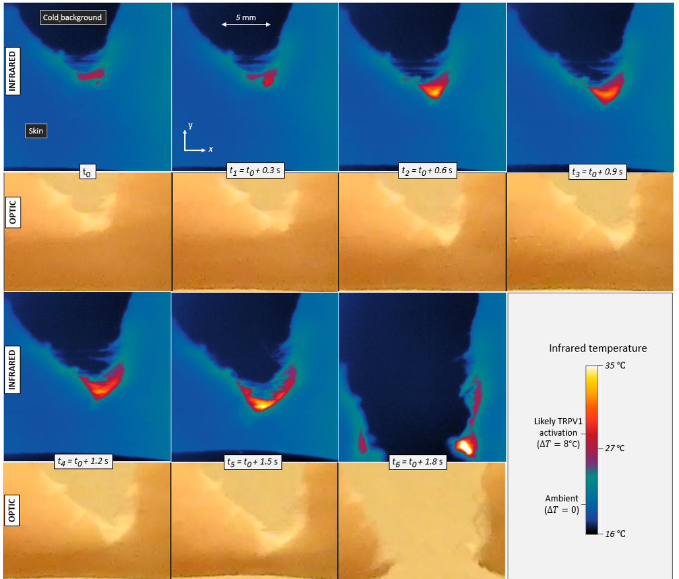
FIG. 3. Infrared temperature maps and corresponding optical frames during the propagation of a tensile crack in porcine skin (skin specimen V). Seven different times are displayed with a constant increment in between. The maximum temperature elevation is \Delta T = 8^\circ\text{C} in the first frame ( t_0 ) and up to \Delta T = 17^\circ\text{C} in the last one ( t_6 ). Contrarily to the infrared camera, the optical camera monitored the whole set-up and was not equipped with a macroscopic lens, hence the noticeable difference in image resolution. It also recorded the skin with a slightly different (non-orthogonal) line of sight, as per Fig. 1.
