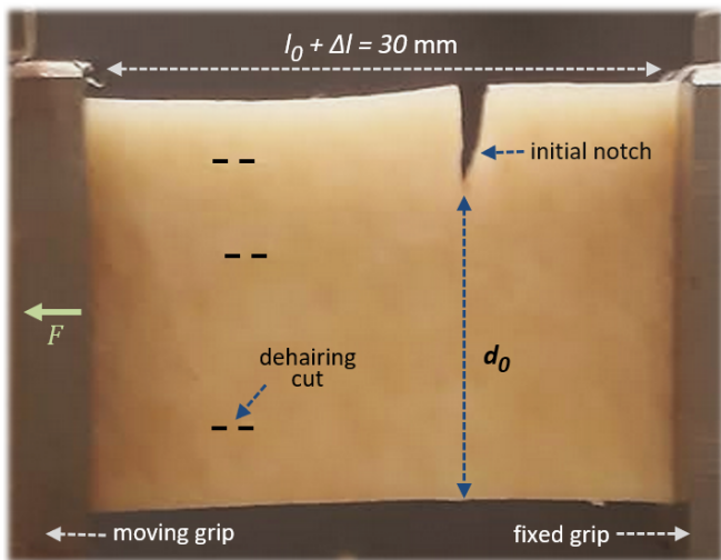
FIG. 2. A porcine skin sample installed in the set-up, with the epidermis facing the camera. A little stretch, \sim 5\% , is here applied by the force F , so that the nominal sample length between the grips is l_0 = 28.5 mm and the stretch is \Delta l = 1.5 mm. The initial unbroken width is denoted d_0 . The dashed lines illustrate some barely visible (shallow) cuts on the epidermis, from the dehairing process. The picture's point of view corresponds approximately to that of the infrared camera during the experiments.
