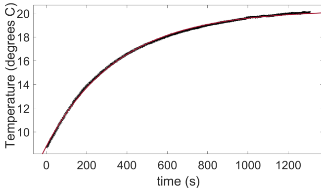
FIG. 8. Warming up in air at room temperature of a skin sample taken out from a refrigerator. The data points (crosses) are measured with the infrared camera. The plain line is a fit of Eq. (B1) with a time constant \tau_a = 356 s.
