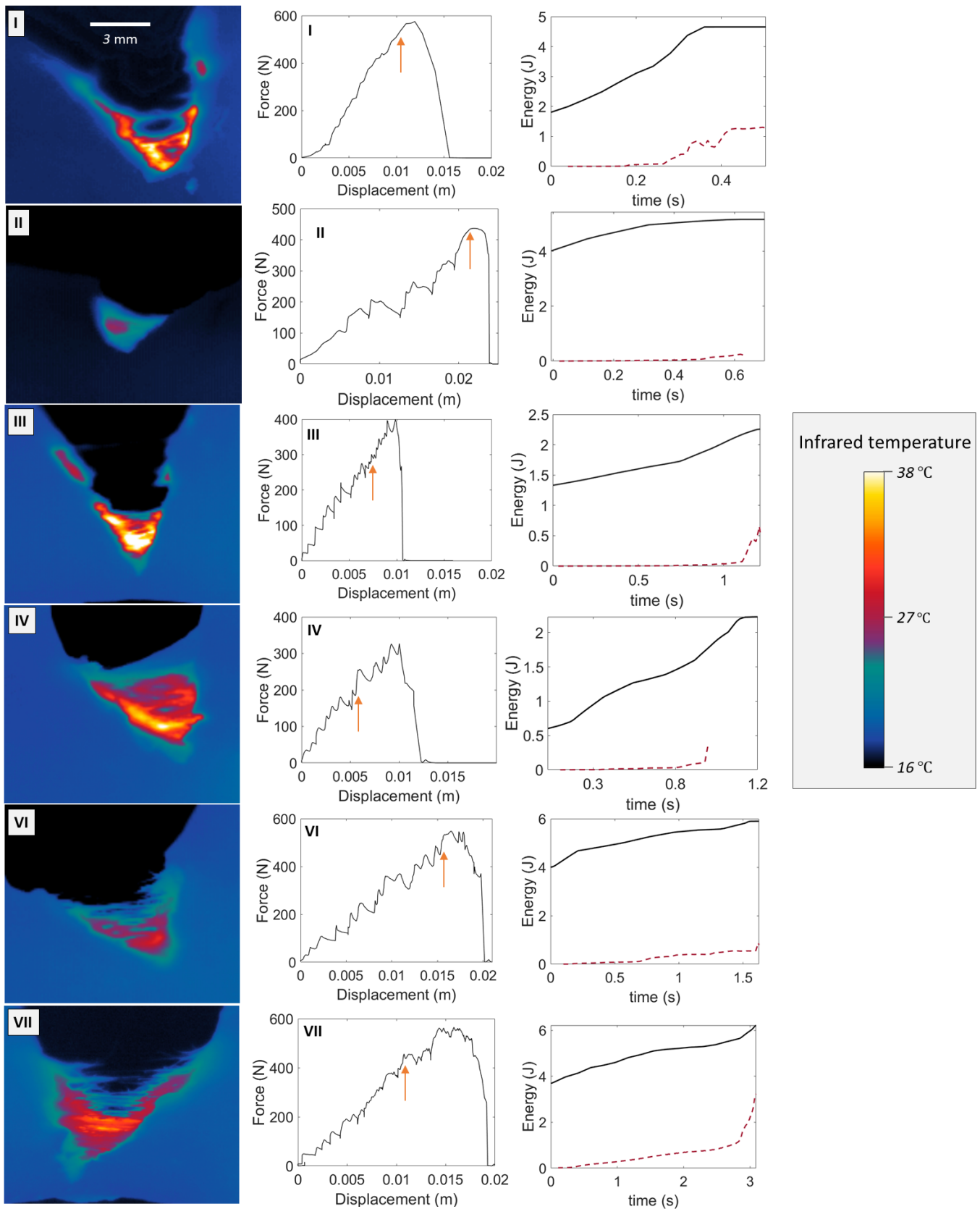
FIG. 7. Temperature map examples (first column), force versus displacement curves (second column) and time evolution of W and U (plain and dashed plot respectively, third column) from the onset of the rupture (arbitrarily at t = 0 s) for skin specimens I, II, III, IV, VI and VII. The arrows on the F versus \Delta l plots indicate the onsets of rupture.
