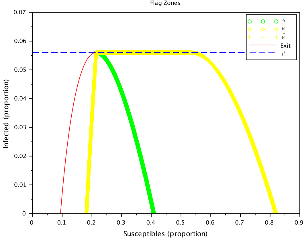
Figure 3: Modified \tilde{\mathcal{Y}} and the outer pointing trajectory at \frac{\gamma}{\beta} .
