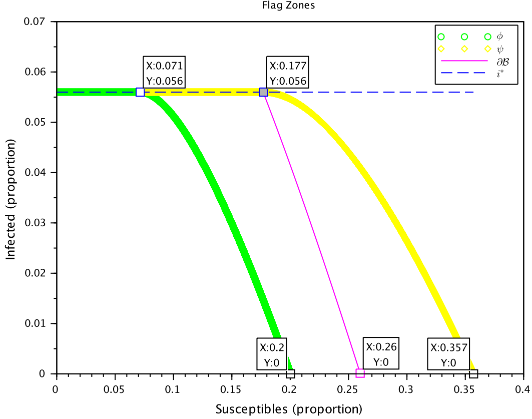
Figure 2: Flag zones for Example 4: N = 67M , I^* = 3.75M , \beta = 1.01 , 1 - \bar{a} = 40\% , \gamma = \frac{1}{14} .
