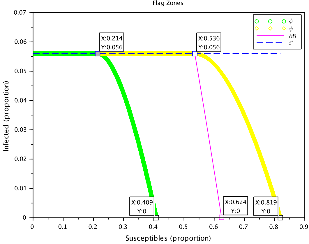
Figure 1: Flag zones for Example 4: N = 67M , I^* = 3.75M , \beta = \frac{1}{3} , 1 - \bar{a} = 40\% , \gamma = \frac{1}{14} .
