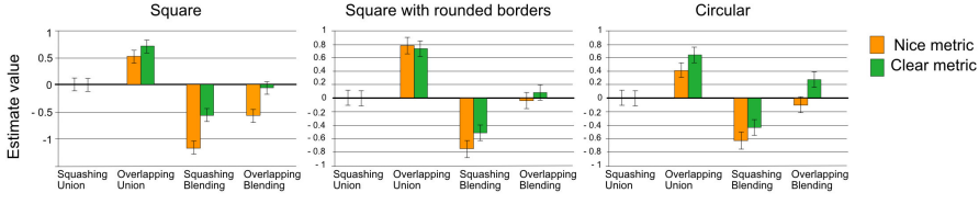
Fig. 6. Results for the pair comparisons between deformers for each decal shape (the y-axis represents the mean rating with respect to Squashing-Union, whose value is always equal to 0). Orange bars show the results for the Nice metric and green bars for the Clear metric.
