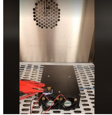
Fig. 8. Junction temperature measurement set up; the diode is mounted on a cooler via a thermal paste and is inserted inside a thermal conditioner.
