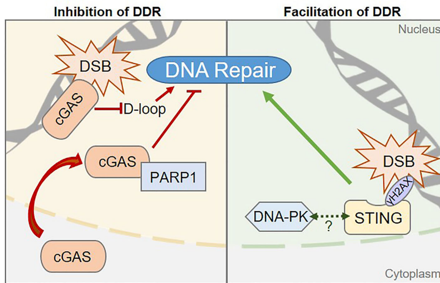
FIGURE 2 | Pattern Recognition Receptors are involved in regulating DNA damage repair processes. Left , The cGAS sensor can inhibit DNA Damage Responses (DDR) via two distinct mechanisms in human cells: 1) cGAS inhibits the Homologous Recombination (HR) pathway by preventing displacement loop (D-loop) formation. 2) cGAS-PARP1 interaction impedes the formation of a PARP1-based complex required for HR-mediated DNA repair. Right , STING promotes DDR in human cells through a yet to be elucidated molecular mechanism, but may rely on the control of components of the Non-Homologous End Joining DNA repair pathway, such as the DNA-PK complex. Dashed arrow between STING and DNA-PK represents the reported interaction between the two proteins (19, 68, 78). Whether this interaction is related to STING-associated DDR control is unknown.
