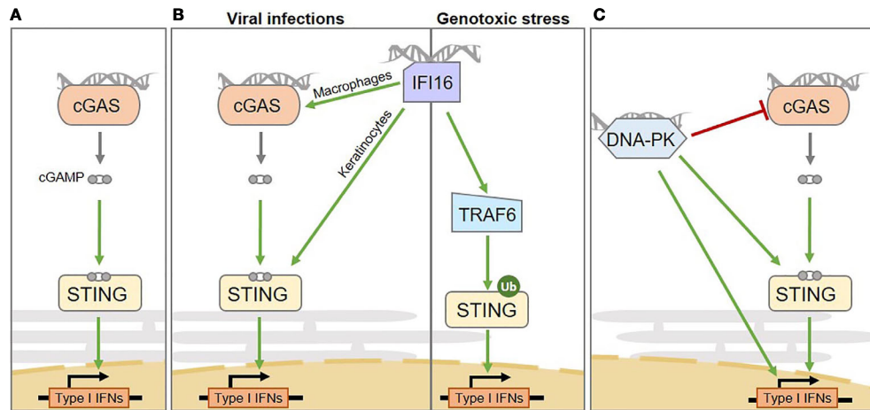
FIGURE 1 | Intertwined cytosolic nucleic acid pathways involved in Interferon and pro-inflammatory cytokine production in human cells. (A) The cGAS sensor activates STING via the production of the cGAMP second messenger. (B) From left to right: the IFI16 sensor mediates inflammation through multiple routes: upon viral infection it activates STING in a cell type-specific manner, either enhancing cGAS-dependent cGAMP production in macrophages or by directly activating STING in keratinocytes; upon genotoxic stress it mediates cGAS-independent, but TRAF6-dependent STING activation. (C) the DNA-PK DNA repair complex was shown to play a role in inducing type I Interferon production upon cytosolic dsDNA detection. However, multiple downstream mechanisms have been proposed, that require STING activation or not, ultimately leading to the phosphorylation of transcription factors responsible for type I Interferon production. The catalytic subunit of the DNA-PK complex (DNA-PKcs) can also suppress cGAS enzymatic activity, by promoting its phosphorylation. IFNs, Interferons.
