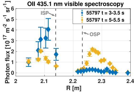
Figure 9: Visible signal of OII 435.1 nm line during the two considered time intervals.
