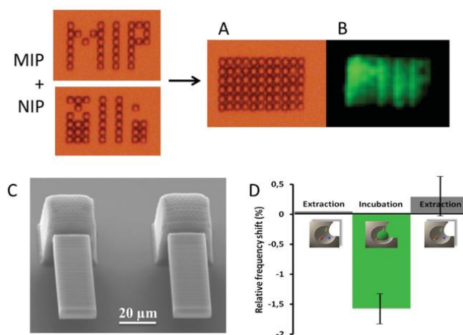
Figure 14. (A–B) Multiplexed NIP and MIP dots polymerized on the same sample by two-photon stereolithography (TPS): (A) Optical and (B) fluorescence microscopy images after binding of dansyl-L-Phe. (C) SEM images of MIP cantilevers fabricated by TPS. (D) Relative frequency shift
