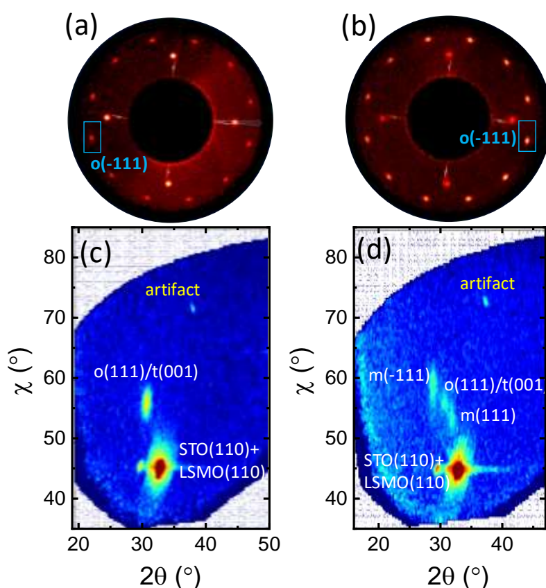
Figure S3. XRD pole figures of (a) \text{ZrO}_2 and (b) \text{Hf}_{0.5}\text{Zr}_{0.5}\text{O}_2 films. The integrated 2\theta - \chi slices around the (001)-oriented phase of (c) \text{ZrO}_2 and (d) \text{Hf}_{0.5}\text{Zr}_{0.5}\text{O}_2 films.
