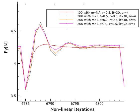
Figure 13. Influence of the a factor on the FSI2 test case. 100 (S-SYN-PF), 200 (P-SYN-PF-PS).
