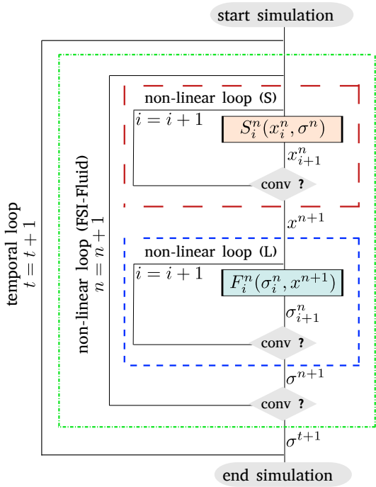
Figure 1. Implicit external algorithm.
