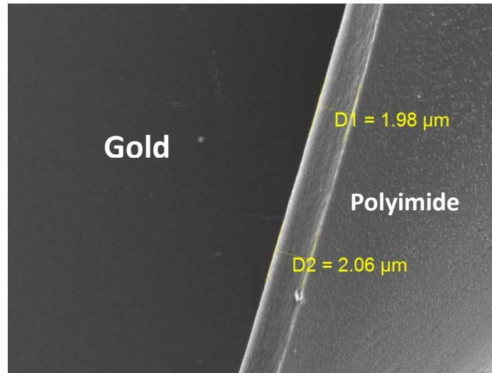
Figure 3. SEM image of a polyimide film deposited on gold surface.
