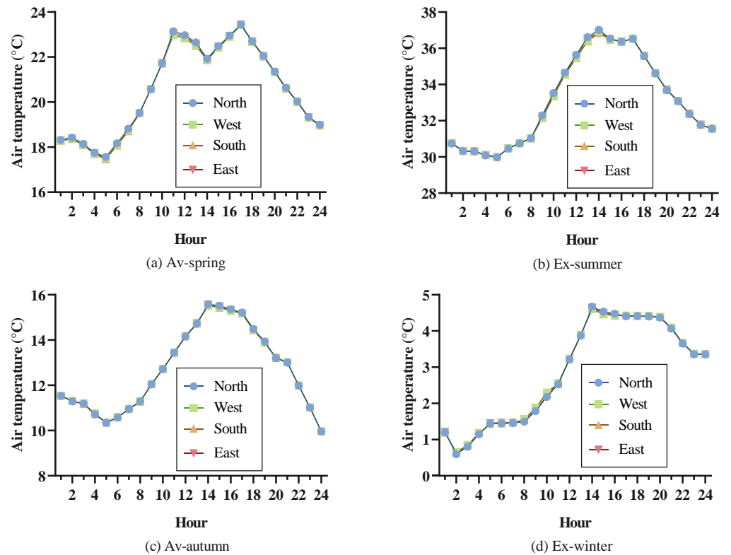
Figure 14. Air temperature of the four orientations at the height of 3 m for the four representative days.
