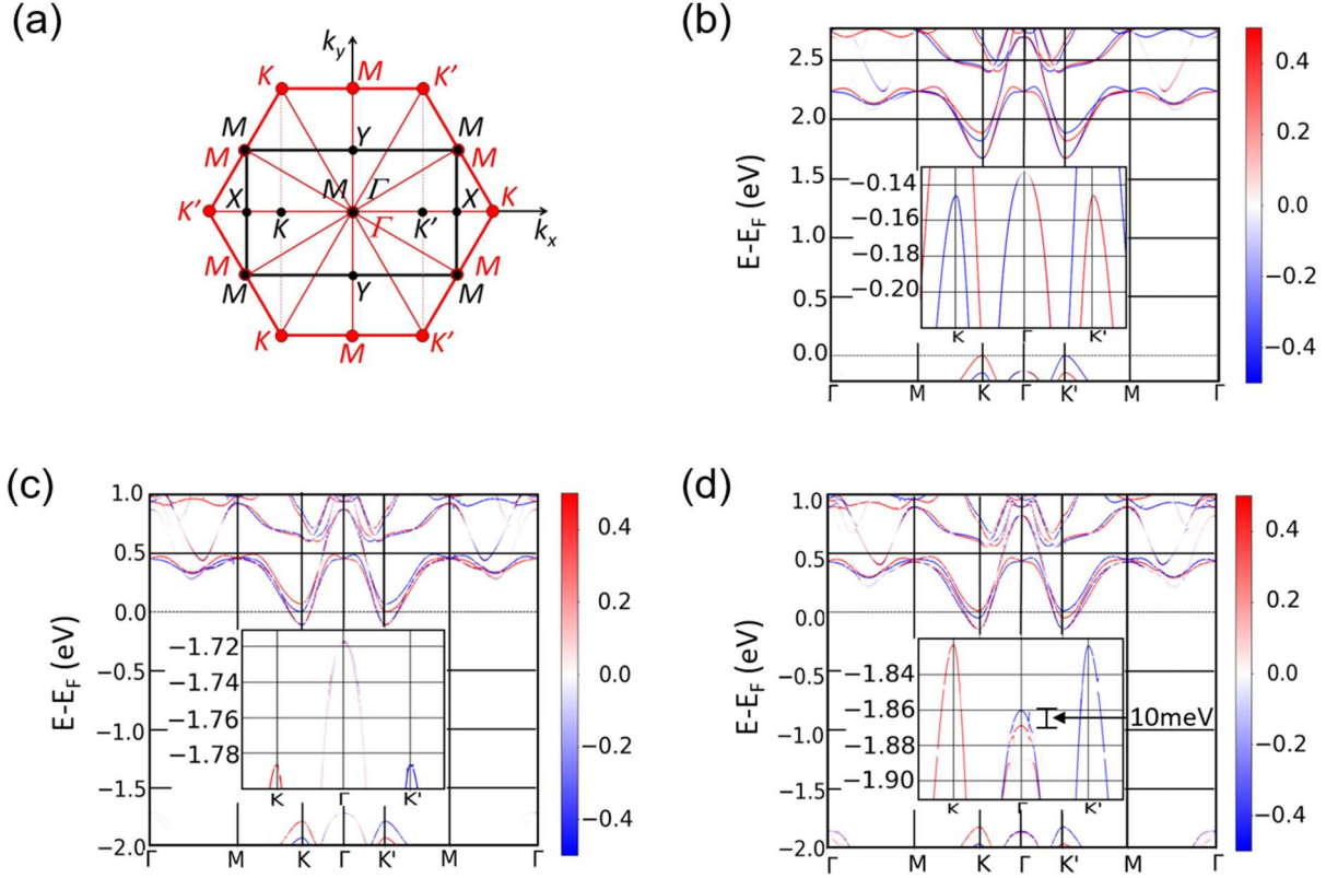
Figure 6: Band structure of the MoS 2 ML in the multilayer structure. (a) Brillouin zone of the unit cells. The red lines represent the hexagonal Brillouin zone of the primitive unit cell of the MoS 2 ML. The black lines represent the rectangular Brillouin zone of the multilayer structure. (b) Band structure of monolayer MoS 2 calculated with a conventional rectangular unit cell. Inset: Magnified valence band structures. The color bar shows the value of the spin-component s_z for each of the Bloch states forming these bands. (c,d) Contribution of the MoS 2 layer to the band structure of the multilayer with (c) 7 MLs of MgO and (d) 3 MLs of MgO. The red and blue lines respectively show the positive and negative values of the spin projection s_z (in units of \hbar ). Insets: Magnified valence band structures show a neglectable Zeeman splitting for 7 MLs of MgO but a large splitting of 10mV at \Gamma point for 3 MLs of MgO.
