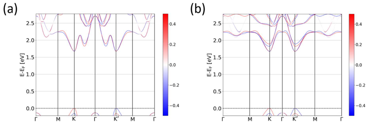
Figure S5: (a) Band structure of a MoS 2 monolayer calculated with a primitive hexagonal unit cell. (b) Band structure of a MoS 2 monolayer calculated with the conventional rectangular unit cell.
