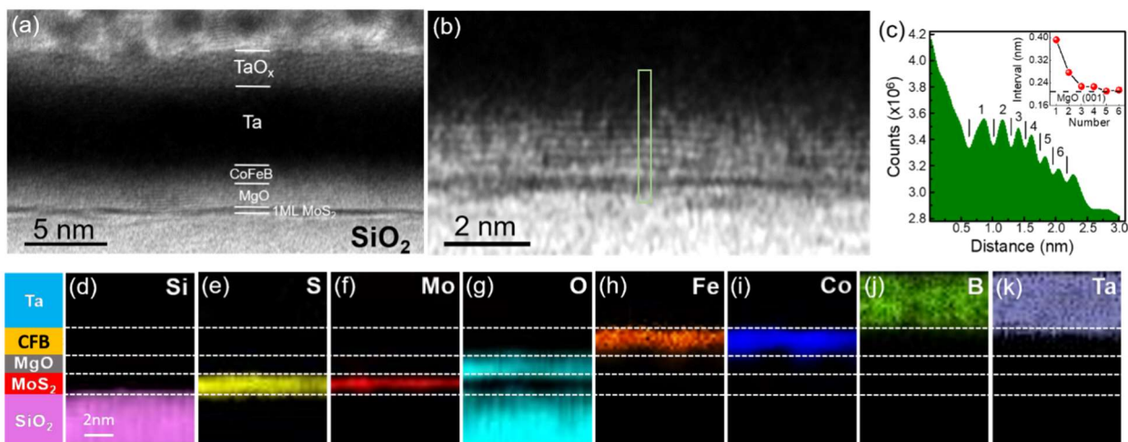
Figure 2: Interfacial structure and chemical characterization of the Ta/CoFeB/MgO/MoS 2 heterostructure. (a) Large scale HR-STEM bright field image showing the multilayer structure. (b) Enlarged image showing the crystallization of MgO on MoS 2 . (c) Integrated intensity profile along the green area in panel (b). Inset: Distance separating two successive oscillation minima as a function of the interval number. (d-k) Chemical maps drawn by processing EELS spectrum images using the signals of (d) Si L3 (99 eV), (e) S L3 (165 eV), (f) Mo M5 (227 eV), (g) O K (532 eV), (h) Fe L3 (708 eV), (i) Co L3 (779 eV), (j) B K (188 eV) and (k) Ta N5 (229 eV) edges, respectively.
