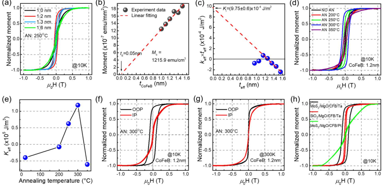
Figure 3: Magnetic characterization of Ta/CoFeB/MgO/MoS 2 heterostructures. (a) Out-of-plane M - H curves for samples with different CoFeB thicknesses with T_{\text{an}}=250^\circ\text{C} measured at 10K. (b) Extrapolation of CoFeB magnetic dead layer t_d from the CoFeB thickness dependent saturation magnetization M_s . (c) t_{\text{eff}} dependence of the product of K_{\text{eff}} and t_{\text{eff}} , where the intercept to the vertical axis of the linear extrapolation corresponds to the interface anisotropy K_i . (d) Out-of-plane M - H curves for the sample with 1.2nm CoFeB before and after different temperature annealing measured at 10K. (e) K_{\text{eff}} as a function of annealing temperature. (f,g) M - H curves for the sample with 1.2nm CoFeB and T_{\text{an}}=250^\circ\text{C} for in-plane and out-of-plane configurations measured at (f) 10K and (g) 300K. (h) Comparisons of out-of-plane M - H curves for three samples: Ta/CoFeB/MgO/MoS 2 , Ta/CoFeB/MgO/SiO 2 and Pt/CoFeB/MgO/MoS 2 . All samples have the same CoFeB thickness and were annealed at 300°C.
