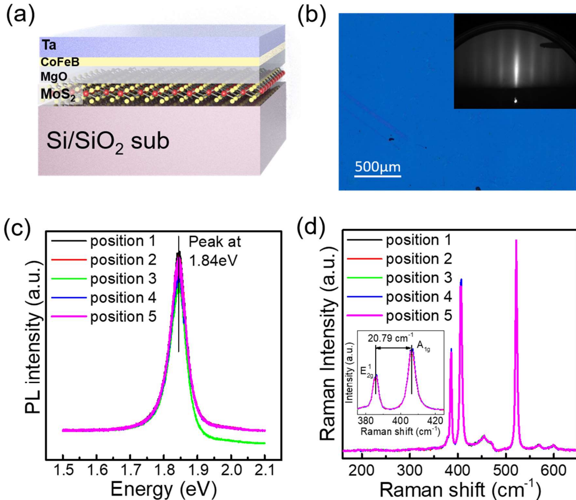
Figure 1: Schematic structure of the investigated sample and characterization of the MoS 2 ML. (a) Schematics of the Ta/CoFeB/MgO/MoS 2 stack on Si/SiO 2 substrate. (b) Large scale optical microscopy image of the surface of monolayer MoS 2 . Inset: RHEED pattern of the MoS 2 surface after annealing at 150°C for one hour. The pattern does not change with different angles of incident e-beam. (c) Room temperature photoluminescence spectra taken on different positions of the MoS 2 ML surface. (d) Raman spectra taken on different positions of the MoS 2 ML surface. Inset: Enlarged spectra showing the distance between E_{2g}^1 and A_{1g} modes.
