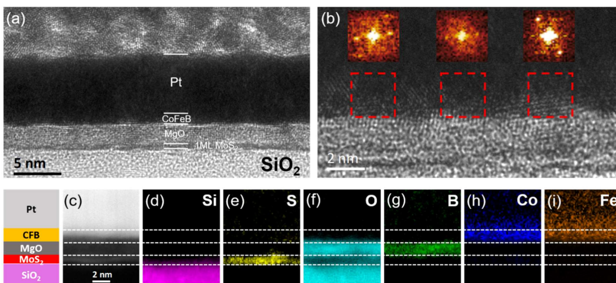
Figure 4: Interfacial structure and chemical characterization of Pt/CoFeB/MgO/MoS 2 heterostructure. (a) Large scale HR-TEM image showing the multilayer structure. (b) Enlarged image showing the crystallization of CoFeB on MgO. Inset: FFT patterns showing that the CoFeB is characterized by polycrystalline features (here 3 different orientations for very close zones). (c) STEM HAADF image of the zone where EELS analyses are performed. (d-i) Element maps drawn from STEM-EELS spectrum image, respectively for (d) Si K , (e) S L , (f) O K , (g) B K , (h) Co L and (i) Fe L edges.
