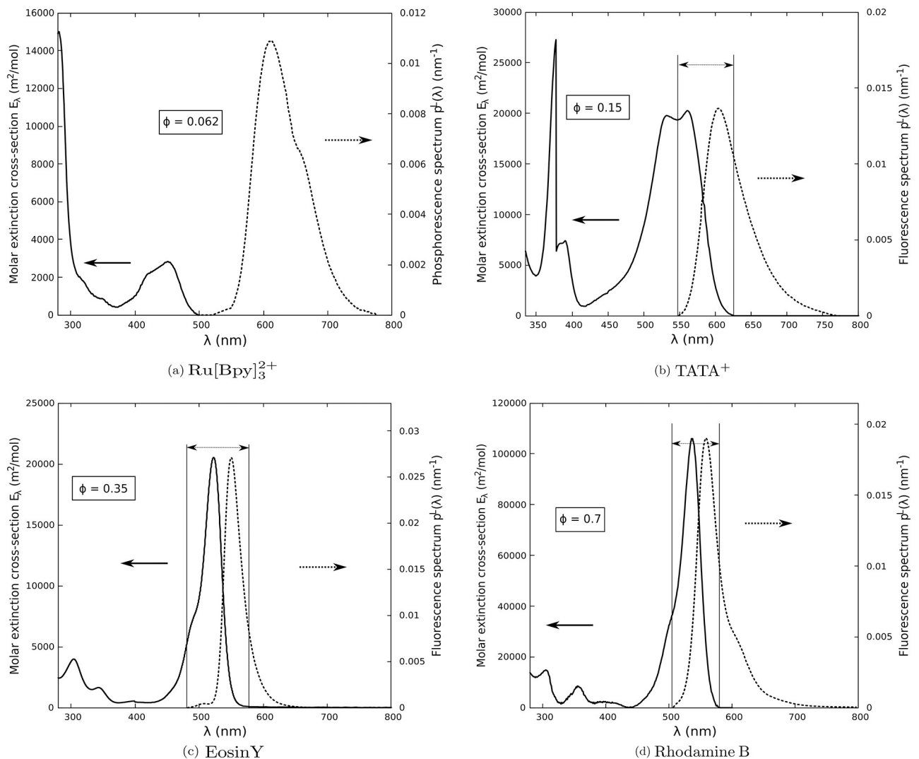
Fig 2. Photosensitizer radiative properties. In all plots, plain lines stand for UV-visible molar extinction cross-section spectrum E_\lambda and dashed lines for luminescence emission spectrum p^l(\lambda) . Luminescent quantum yield \Phi is provided in a box. (a) Ru[Bpy] 3 Cl 2 (40 \mu M) in aqueous buffer (pH 6.8) solution [48]. (b) TATA(Cl) (0.5 mM) UV-visible molar extinction cross-section, TATA(Cl) (10 \mu M) fluorescence emission spectrum and quantum yield under argon in acetate buffer (1 M) at pH 4.5 [25] (c) Eosin Y (24 \mu M) in a mixture of triethylamine (10% vol.) in water at pH 10.5 [18, 21] (d) Rhodamine B in ethanol [26, 49]. Extinction cross-sections are obtained assuming that absorbance A_\lambda measured by the authors cited above using spectrophotometry experiments can be interpreted as A_\lambda = 1 - \exp(-E_\lambda CL) . Overlapping between molar extinction cross-section and luminescence emission spectrum is represented for each photosensitizer (except Ru[Bpy] 3 Cl 2 for which no overlapping is observed) by 2 parallel lines linked by a double arrow.
