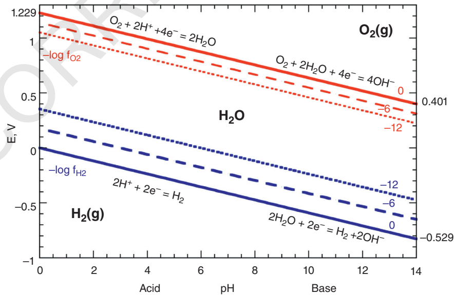
Figure 1.1 E-pH diagram reporting the stability of water at T = 25°C and P = 1 bar for different partial pressure of H 2 and O 2 reported as log f O 2 values.
