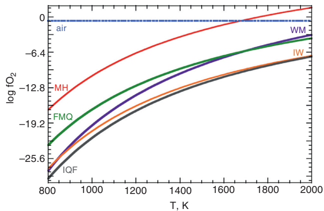
Figure 1.6 Common solid oxygen buffers used in petrology and geochemistry. The lines represent the fugacity-temperature conditions where the phases coexist stably. FMQ: fayalite, magnetite, quartz; IW: iron-wüstite; WM: wüstite-magnetite; HM magnetite-hematite. Oxygen fugacity values were computed for a total pressure of 1 bar (solid lines). Also reported is the value of \log f_{\text{O}_2} in air ( \text{PO}_2 \sim 0.21 bar).
