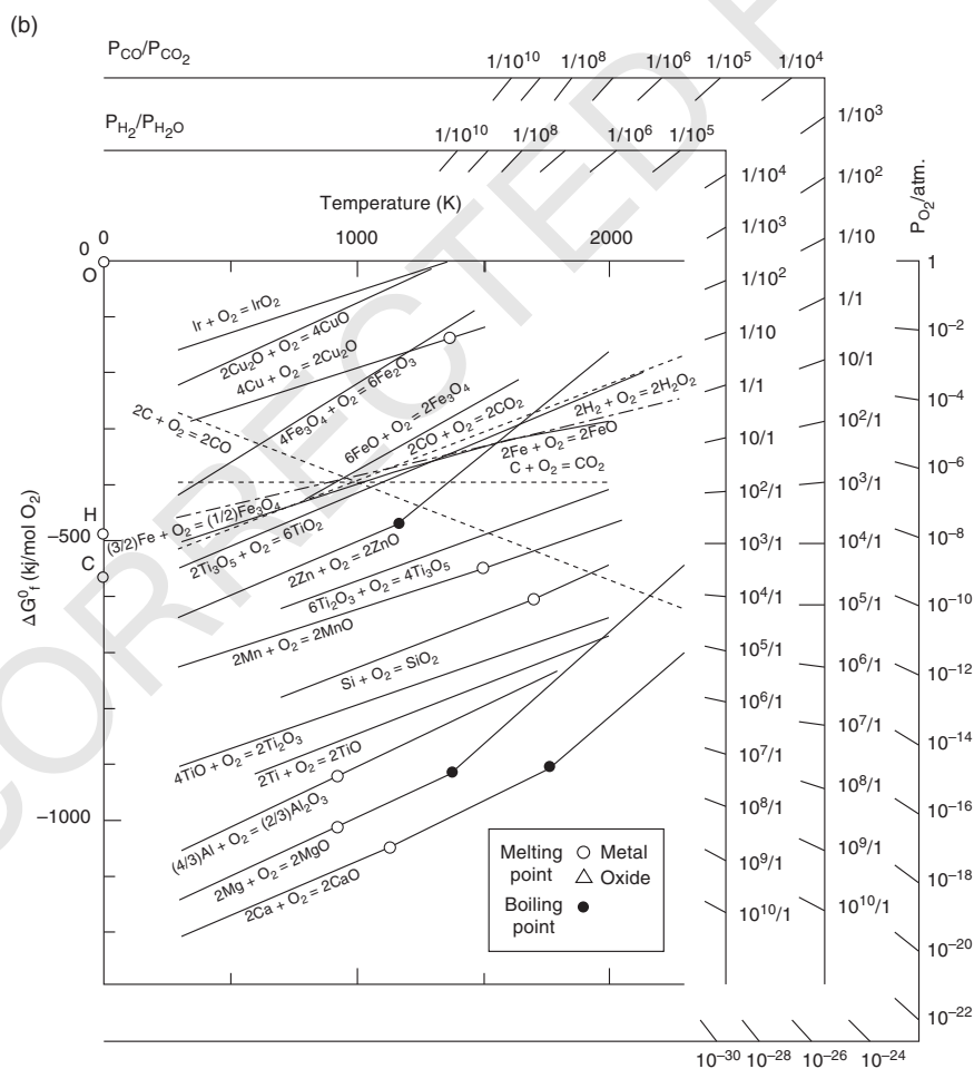
Figure 1.5 (a) Ellingham diagram for the main components of the slag (solid lines) and possible reducing agents (dotted lines). The slopes of the lines representing \Delta G_f^0 - T relations change at the temperature in which the phase transformations of reactants or products occur. Modified from Zhang et al. (2014). (b) Full Ellingham diagram for some relevant oxides including \text{CO}_2 equilibria and normographic scales for oxygen fugacity and related quantities via \text{CO}/\text{CO}_2 and \text{H}_2/\text{H}_2\text{O} ratios at P_{\text{tot}} = 1 bar. The scale of \text{P}_{\text{H}_2}/\text{P}_{\text{H}_2\text{O}} ratio is used in the same manner as that of \text{P}_{\text{CO}}/\text{P}_{\text{CO}_2} ratio, except that the point H on the ordinate at T = 0 K is used instead of point C. Modified from Hasegawa (2014). All reactions' components are considered in their pure stable phase at 1 bar and T of interest.
