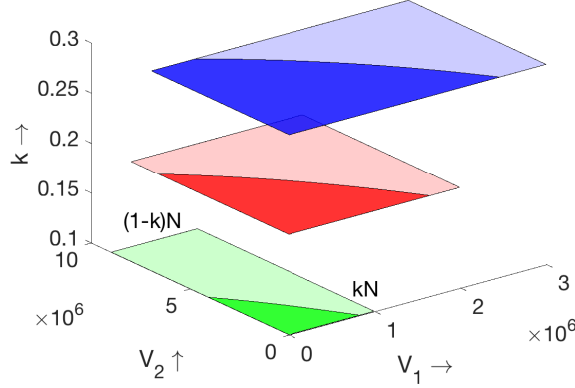
Figure 1: Regions of epidemic growth and extinction are marked with deep and light colours, respectively. Parameter values are \beta_{11} = 4, \beta_{22} = 1, \beta_{12} = \beta_{21} = 2.5, \sigma_1 = \sigma_2 = 1 and k = 0.1 (green), k = 0.2 (red) and k = 0.3 (blue).
