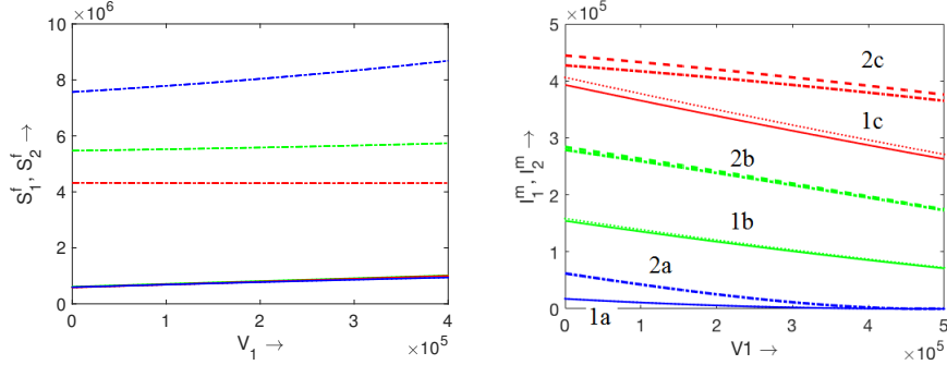
Figure 2: Left panel: the final sizes of epidemic for two groups S_1 (solid lines) and S_2 (dashed lines) for k = 0.1 (blue), k = 0.2 (green), k = 0.3 (red). Note that analytical and numerical results coincide. The final sizes for S_1 and different values of k are very close to each other. Right panel: the maximal numbers of infected individuals for two groups S_1 (1a, 1b, 1c) and S_2 (2a, 2b, 2c) for k = 0.1 (blue), k = 0.2 (green), k = 0.3 (red). Each pair of close curves corresponds to the analytical and numerical results. Other parameter values are as follows: \beta_{11} = 4, \beta_{22} = 1, \beta_{12} = \beta_{21} = 2.5, \sigma = 1, V_2 = 2.4 \cdot 10^6 - V_1 .
