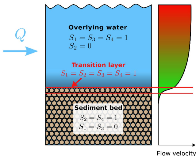
Figure 1. Conceptual description of the domain decomposition with parameters used in Equation 1 for the three layers configuration.
