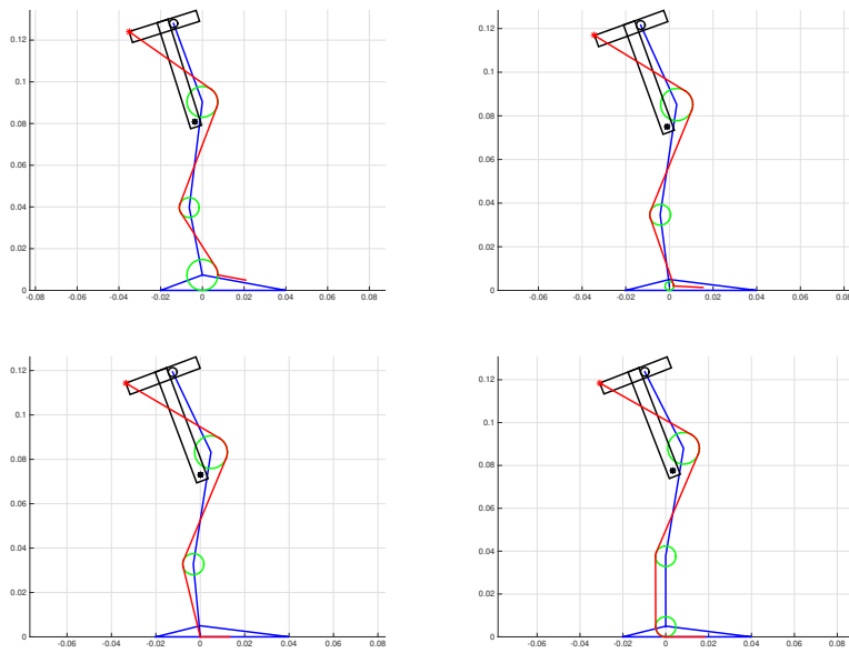
Figure 10: Several equilibrium configuration for different value of the dimension of the finger pulley and different way the cable pass around the pulley. In the upper left case, the pulley of the knee and finger have the same size, the knee is at the vertical of the finger joint. In the upper right case, the case studied. In the lower left case, the pulley has 0 diameter, the angle of the foot as no influence on the cable length, the CoM is projected at the finger joint. The lower right case, the foot is vertical.
