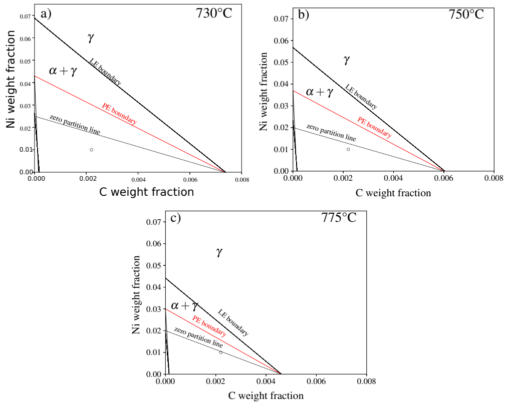
Figure S3: Isothermal sections of the Fe-C-Ni at a) 730°C, b) 750°C and c) 775°C showing the different possible growth modes (LEP-LENP and PE) for the studied compositions (grey circles).
