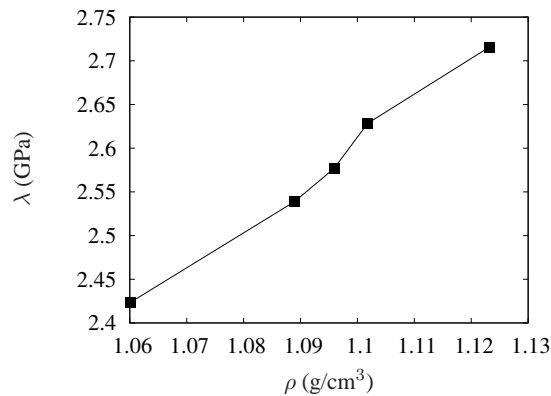
FIGURE 3 – Lamé's first coefficient vs density measured on alginate beads of various concentration in alginate
