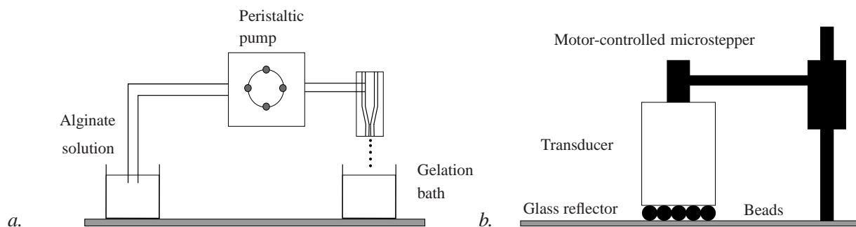
FIGURE 1 – Experimental setups for a. the fabrication of alginate beads by extrusion and b. the acoustic wave measurement by a pulse-echo method.
