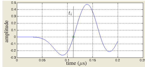
FIGURE 2 – Time-average ultrasonic signal received by the transducer in position z_i ( i = 1, 2 ) after transmission through a single layer of alginate beads and reflection on the bottom plane. We choose to compare the difference between the times of the first zero-crossing, t_i . This time difference corresponds to the time during which the ultrasound travels the distance 2(z_1 - z_2) .
