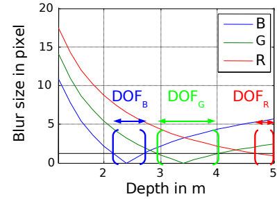
Fig. 8. Illustration of the image quality criterion generalized depth of field (GDOF): the union of the R,G,B depth of fields (DOF). Note that in this example, the GDOF does not stand within a single continuous depth range.
